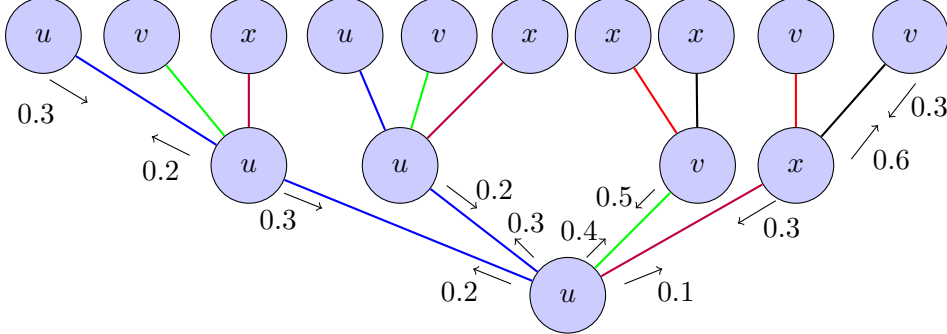
Figure 2: the first levels of the universal cover of \mathcal{G} in Figure 1 (not all weights are on the picture), rooted at u . Note that two non-backtracking paths start from u , since the blue edge in \mathcal{G} gives rise to two oriented edges opposite to each other.
