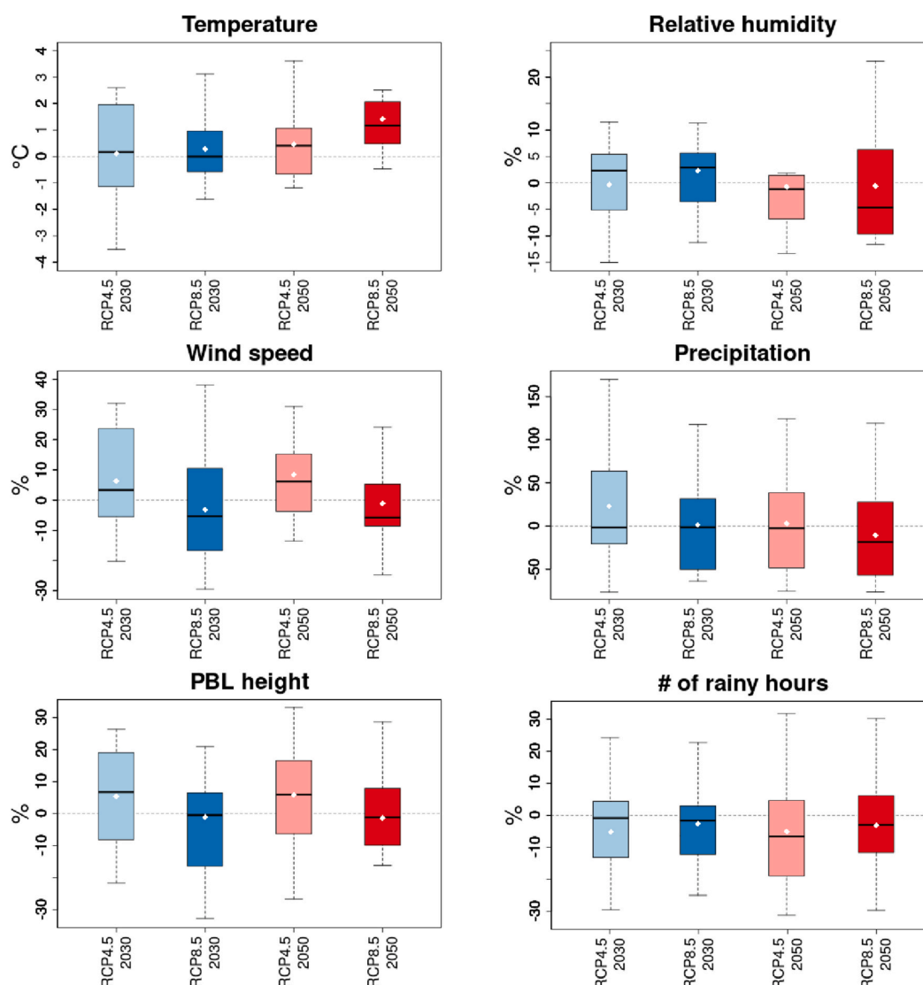
Fig. 5. Changes of meteorological parameters in future scenarios compared to historic simulation for 2005. The values are shown in percentage, except for temperature for which the delta in ^{\circ}\text{C} is shown. The boxplots are standard boxplots, the white spot on each boxplot shows the average for each one, the name of the scenarios is given on the x-axis of each grid. The dotted line shows the 0 reference.
