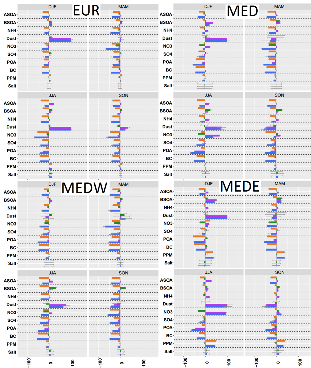
Figure S18.1. Seasonal relative impact of climate, BC and emission drivers on PM_{10} components for different sub-domains, the name of the sub-domains is written on each panel. Each sub-panel shows one season. Error bars show the confidence interval calculated by annual averages.
