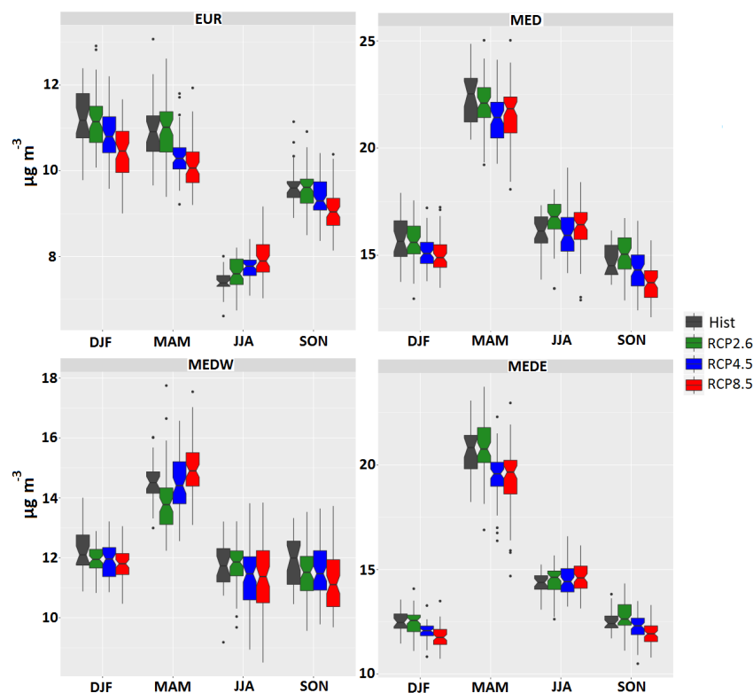
Figure 6. Seasonal box plots for all scenarios for all seasons for PM_{10} (historic simulations are black, RCP2.6 is green, RCP4.5 is blue and RCP8.5 is red) for the different subdomains. Scales are different for different subdomains.
