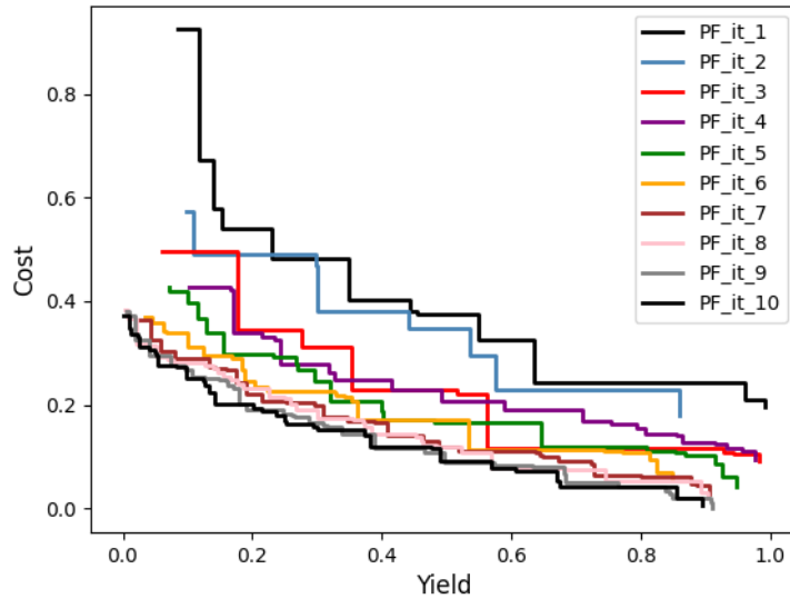
Figure 6.8: Comparison of the Pareto fronts of the 10 iterations of our EPFAM process.
