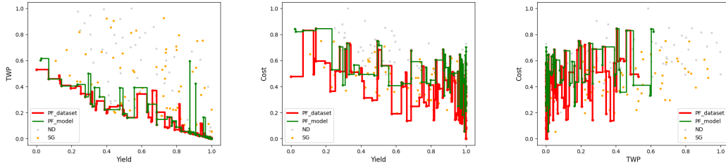
Figure 6.10: Scatter plots of the EPFDM best model with HV_{dev} showing the pair-wise relationship between objectives.
