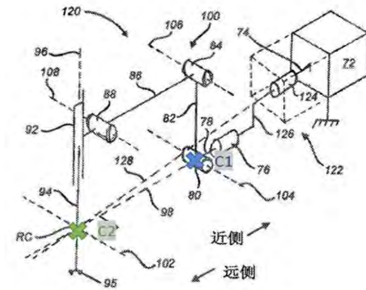
FIGURE 4.26 – Architecture du robot Da Vinci, Intuitive Surgical Inc.
