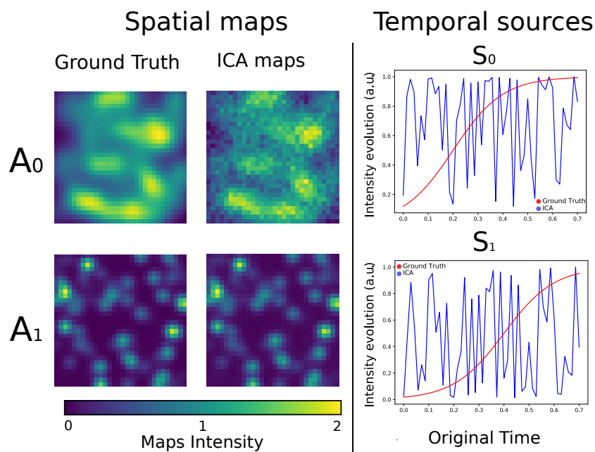
Figure 2.13: Spatial maps: Sample slice from ground truth images ( A_0 \lambda = 2 mm, A_1 \lambda = 1 mm), the maps estimated by ICA. Temporal sources: Ground truth temporal sources (red) along with sources estimated by ICA (blue).
