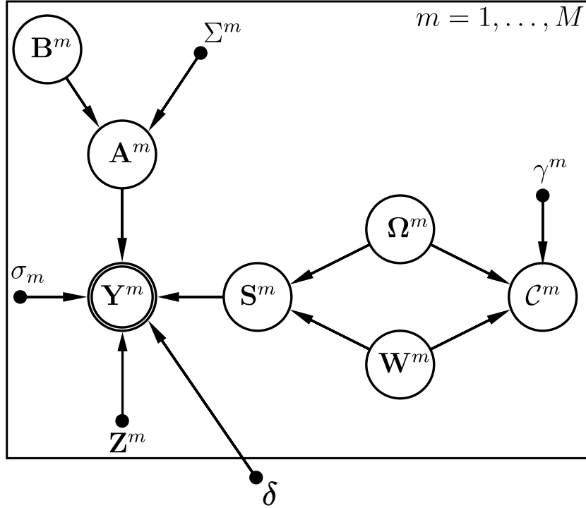
Figure 2.2: Graphical model for imaging data, Y = \{Y^m\} .
