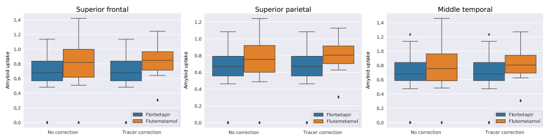
Figure 4.2: Distribution of the regional amyloid uptake depending on the tracer used during acquisition for the subjects from the GMC cohort. 76 amyloid-PET scans were acquired using florbetapir and 17 using flutemetamol. Tracer correction indicates that the regional amyloid uptake of subjects whose PET scan was acquired using flutemetamol was converted to a florbetapir scale. GMC: Geneva Memory Center; SUVR: Standardized Uptake Value Ratio; PET: Positron Emission Tomography.
