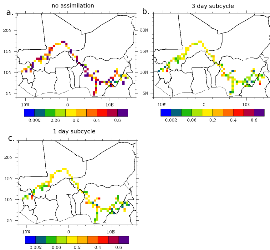
Figure 4.5: Relative error of water levels (m) averaged over the period of assimilation. Errors are reduced for both the 1 and 3 day sub-cycle orbits (Pedinotti et al., 2014).
