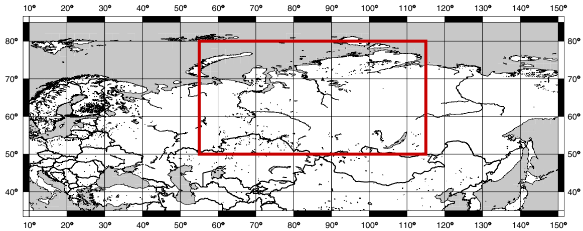
Fig. 1. The Siberian study domain is enclosed within the boxed region.
