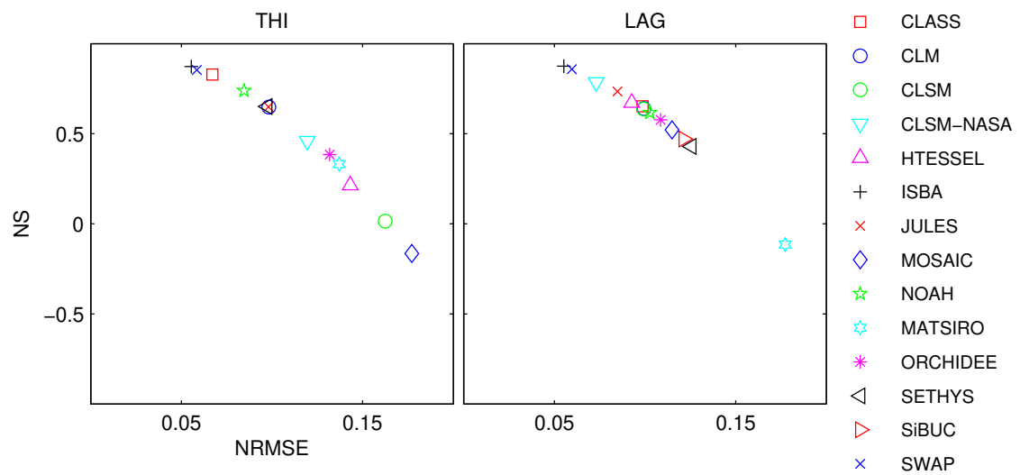
Figure 3.10: Best objective functions resulting from optimization runs for experiments using Thiessen (THI) and kriging-Lagrangean (LAG) based precipitation products. NS represents the Nash-Sutcliffe statistical metric, and NRMSE represents the normalized root mean square error: statistics are for the entire period and computed at the river outlet at B  teroux (Getirana et al., 2017).
