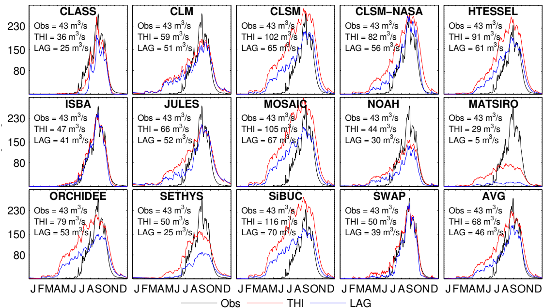
Figure 3.9: Daily discharge annual cycle (averaged from 2005-2008) at the Bétérou station ( \text{m}^3 \text{s}^{-1} ) for each LSM after routing using ARTS. The average discharge is shown for the observations (Obs), and simulated for the THI and LAG input rainfall data (Getirana et al., 2017).
