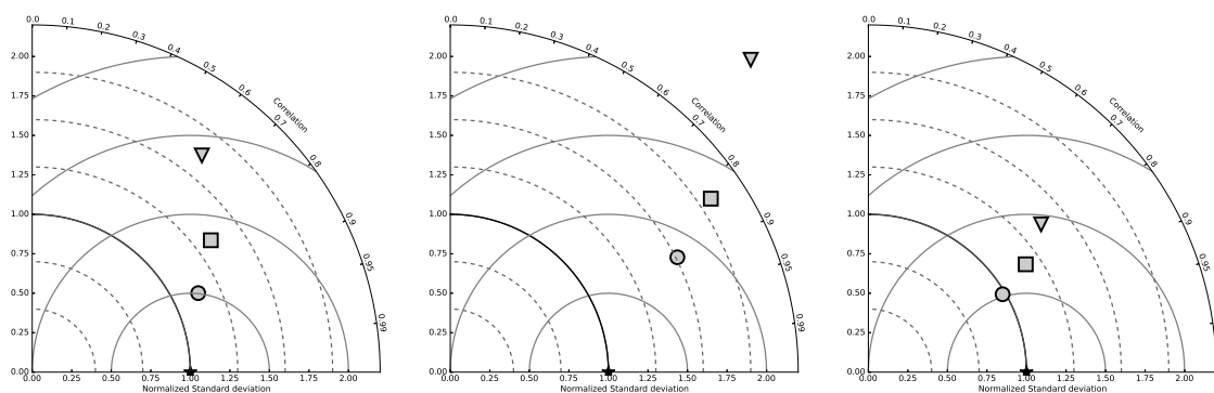
Figure 2.4: Ground heat flux plotted on Taylor diagrams for (from left to right) for the LeBray, Puéchabon and Barbeau sites. The points correspond to ISBA (composite: triangle), ISBA-MEB (square) and ISBA-MEB-L (circle).
