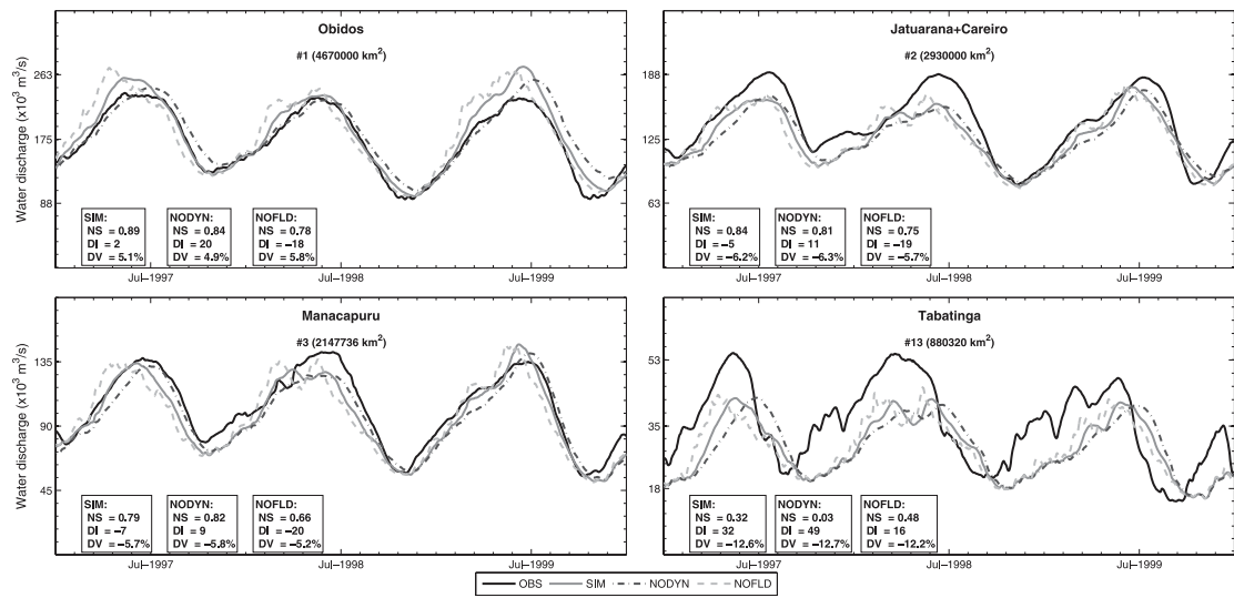
FIG. 16. Hydrographs at four gauging stations along the Solimões–Amazon River (Obidos, Jatuarana+Careiro, Manacapuru, and Tabatinga) resulting from experiments evaluating effects of floodplain dynamics on water discharges.
