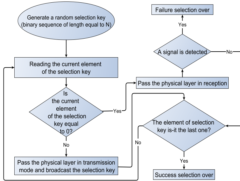
Figure 4.4: Active signaling
