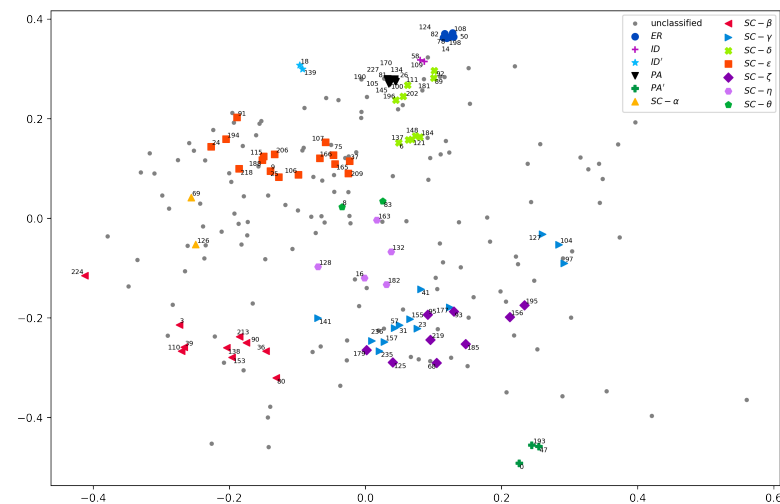
Figure 2: Network generators mapped on a two-dimensional layout according to their pairwise distances. Colors and shapes indicate generator families manually identified as semantically similar. ER means Erdos-Rényi (i.e., a uniformly random process reconstructs well the empirical network), PA means preferential attachment, ID means a very simple process proportional to node IDs. In particular, “SC” generators (for Social Circle) involve a notion of node class and are over-represented in Facebook friendship networks. See Menezes and Roth (2019a) for details.
