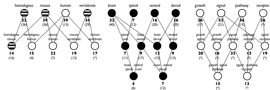
Figure 11: Evolution of the socio-semantic macro-structure of the zebrafish community from the period 1990-95 to 1998-2003, using pruned socio-semantic lattices focused on the top (most generic and populated) ECs. Each node is an EC labeled with its concept set, and its actor set size as a percentage of the total population. Figures are in bold for 1998-2003 and in italics and inside brackets for 1990-1995, showing the lattice evolution over the period. White and black ECs experienced a marked population increase or decrease (more than 15%), dashed ECs stagnated (less than 15%), stars denote new ECs in 1998-2003. From Roth (2010).
