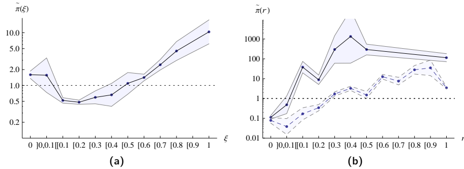
Figure 9: Hypergraphic propensity (team bias): (a) for the proportion of experts per article; (b) for hypergraphic repetition ratios (social in solid line, semantic in dashed line). (Geometrically averaged behavior based on all four datasets.)
