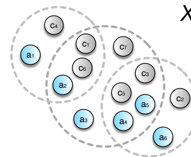
Figure 6: Toy example of a socio-semantic hypergraph X . Nodes represent either agents from S or concepts from \mathcal{S} . The boundaries of three partially-overlapping socio-semantic hyperedges are figured by thick dashes: the top-left hyperedge, for instance, gathers \{a_1, a_2, c_1, c_4, c_6\} .
