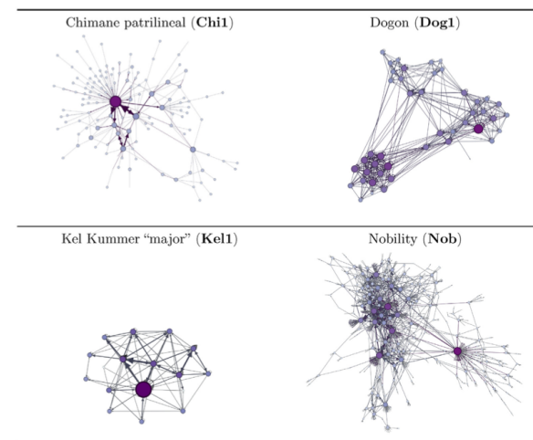
Figure 5: Some empirical alliance networks: node size is proportional to strength, while arrow width is proportional to arc weight (graphs were rendered with GePhi using the ForceAtlas visualization algorithm). From Roth et al. (2013).
