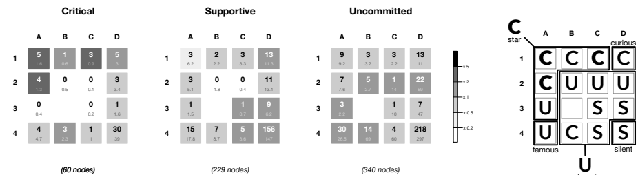
Figure 14: Application of the model of Fig. 13 to a Twitter subspace focused on users discussing the 5th Assessment Report (AR5) of the Inter-Governmental Panel on Climate Change (IPCC). The core is now defined over the most active users, who were manually labeled as supportive, critical, or neutral toward climate change science (Roth and Hellsten, to appear). The three matrices on the left describe how each alignment is more or less present than expected if position did not matter i.e., if it were uniformly represented in each slot. The matrix on the right shows that critical discourse occupies the dominant positions, even if they are the minority.
