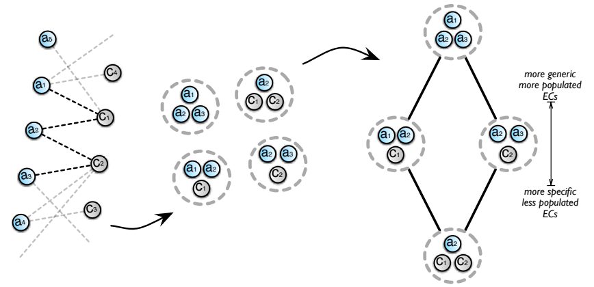
Figure 10: Illustration of the construction of a socio-semantic lattice \mathcal{L} , from left to right: (i) a bipartite graph features usage of concepts c_1, c_2 , etc. by agents a_1, a_2, a_3 (part of \chi ); (ii) maximal groups of agents using the same concepts are then extracted (they are meso-level socio-semantic hyperedges and thus form a type of socio-semantic hypergraph X ) and finally arranged into a hierarchical socio-technical lattice \mathcal{L} (being a high-level socio-semantic hypergraph with the partial order \geq_{ec} ). Note that S and \mathcal{S} are by definition bicliques and respectively upper and lower bounds of all ECs.
