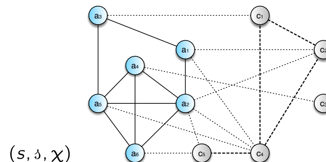
Figure 7: Ontology of a typical socio-semantic network given by the triplet (s, \delta, \chi) i.e., social, semantic, and socsem networks: nodes a \in S denote actors, while nodes c \in \delta denote concepts; links correspond diversely to interaction, co-occurrence, or usage; they may be directed or undirected. This socio-semantic network is not derived from the example of Fig. 6 and illustrates the situation where links of s , \delta or \chi do not configure cliques.
