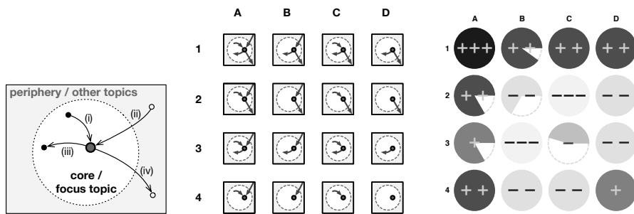
Figure 13: Socio-semantic, or structural-topical model introduced in Cardon et al. (2011, 2014). Left: It relies on a double dichotomy between incoming or outgoing links, internal (white area) or external (gray area) to a topical territory or a core. Middle: From there, 16 cells are defined, depending on whether a node is most connected (e.g., top 20%), or not, in each of the 2x2 categories. Right: It has been applied to French and German blogspaces, for 6 (x2) topical territories (cooking, IT, politics, etc.). Symbols correspond to over- or under-representation (+ or -), weak or strong (+++ vs. +), and are here averaged for all territories (full disks indicate that all territories behave similarly). It exhibits remarkable structural positions which are always over- or under-represented, while some slots, such as C3, exhibit a mixed pattern: they exist only for self-centered topics (home cooking, worn fashion) which are thus truly community-centric territories (as in Rheingold, 1993), not for public space topics (politics, IT progresses).
