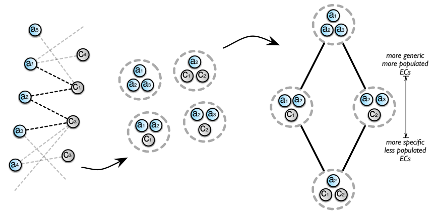
Figure 10: Illustration of the construction of a socio-semantic lattice \mathcal{L} , from left to right: (i) a bipartite graph features usage of concepts c_1, c_2 , etc. by agents a_1, a_2, a_3 (part of \chi ); (ii) maximal groups of agents using the same concepts are then extracted (they are meso-level socio-semantic hyperedges and thus form a type of socio-semantic hypergraph X ) and finally arranged into a hierarchical socio-technical lattice \mathcal{L} (being a high-level socio-semantic hypergraph with the partial order \geq_{ec} ). Note that S and \mathcal{S} are by definition bicliques and respectively upper and lower bounds of all ECs.
