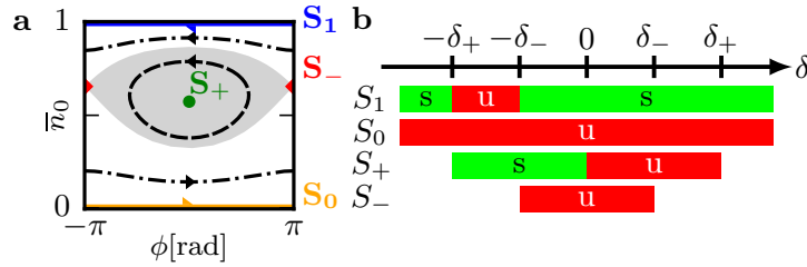
Figure 32: Fixed points of the dissipative spin-mixing model 2. a: Phase space portrait of the stationary solutions of Eqs. (4.24, 4.25). The two limit cycles are labeled S_0 ( \bar{n}_0 = 0 , solid orange line) and S_1 ( \bar{n}_0 = 1 , solid blue line) and the two fixed points S_+ (green dot) and S_- (red diamond). The black lines show typical trajectories in the oscillating (dashed line) or rotating (dash-dotted lines) regimes. The shaded area covers the oscillating regime. The plot is shown for \delta/2\pi = -10 Hz, U_s/h = 25 Hz, \kappa \simeq 0.38 ( \delta_-/2\pi \simeq 32 Hz) and a damping coefficient \beta_2 \rightarrow 0^+ . b: Table summarizing for \beta_2 \rightarrow 0^+ the ranges of detuning where each stationary solution is stable ('s') or unstable ('u'). The boundaries \delta_{\pm} are defined after Eq. (4.33).
