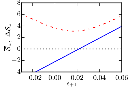
Figure 24: \Delta S_z (dash-dotted red line) and \bar{S}_z (blue line) as a function of the correction factor \epsilon_{+1} ( \epsilon_{-1} = 0 ). The minimum of \Delta S_z and the zero of S_z coincide almost perfectly.
