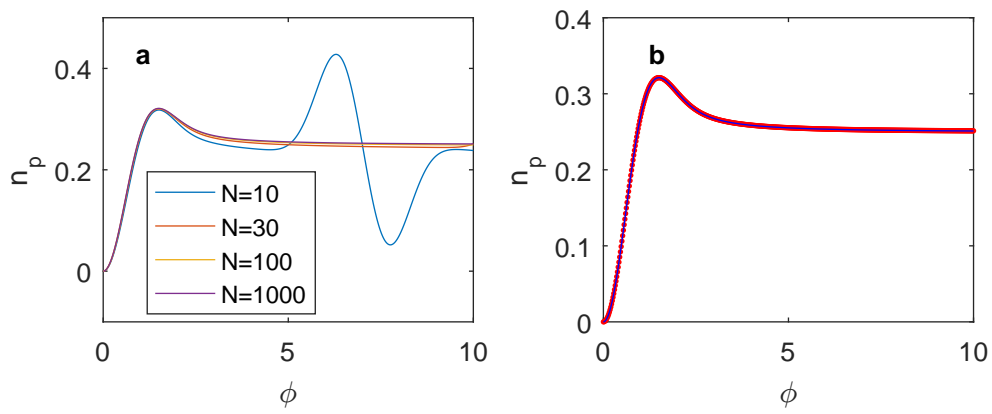
Figure 68: Numerical resolution of the thermalization dynamic of a nematic state at q = 0 . a n_p vs \tau (defined above) for various atom numbers. For small N = 10 we see an early revival of the dynamic. For larger N , we observe thermalization, and we verify the universality of the curve n_p(\tau) . b The blue line is the exact result for N = 1000 atoms, the red dots are the approximate formula derived in this appendix. The error of order 1/N is not visible.
