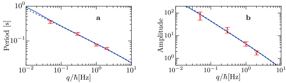
Figure 42: (a) Period and (b) amplitude of the oscillations of N_p versus the QZE q . The solid blue lines are the results of numerical simulation and the black dotted lines are the predictions of the UPA.
