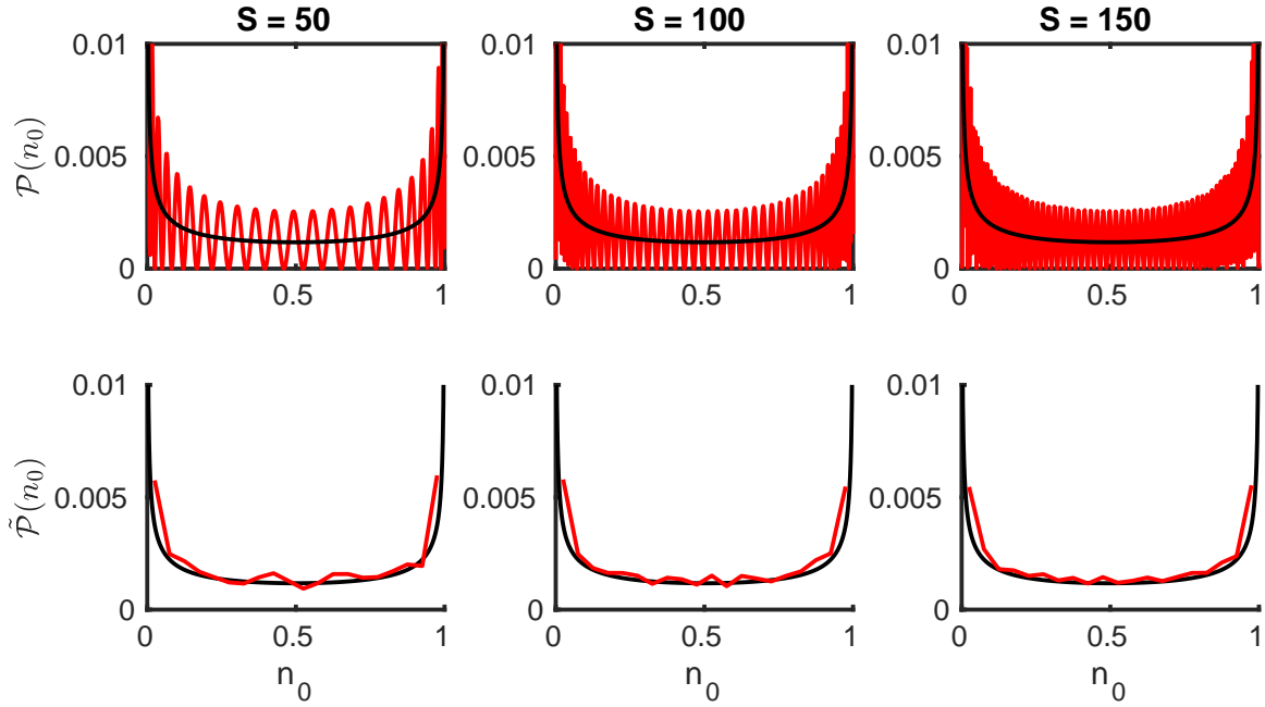
Figure 46: Distribution of the reduced population n_0 in the |N, S, M_z\rangle states, for N = 1000 , S = 50, 100, 150 and M_z = 0 . The upper panels show the exact distributions and the lower panels the coarse-grained distributions. The black line corresponds to the analytical result given by Eq. (6.19).
