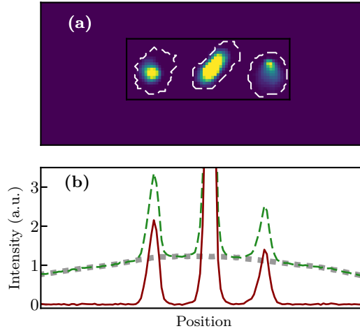
Figure 19: (a) Typical fluorescence image, with optimize ROI (dashed-white line). The hashed region is the ROC used to compute the BRP. (b) Profile before noise removal using the BRP algorithm (green dashed line) and after removal (solid red line). The dotted gray line shows the profile of the BRP.
