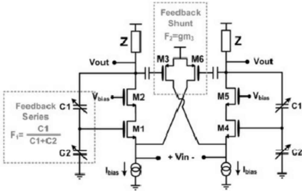
Figure 1.7 – Common gate with two differential feedbacks [8]
