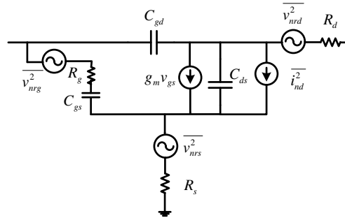
Figure 3.2 – GaAs-pHEMT transistor noise model.
