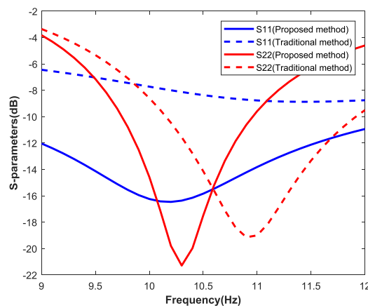
Figure 4.8 – S-parameters of both LNAs
