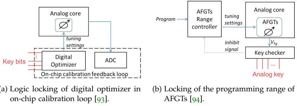
Figure 2.2: Existing locking via the calibration module for analog ICs.
