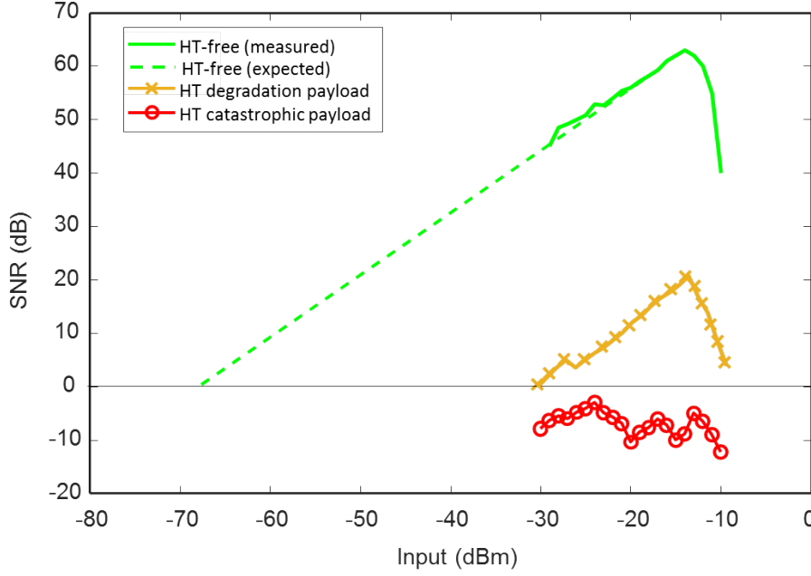
Figure 4.15: Dynamic range under HT-free and HT-infected operation.
