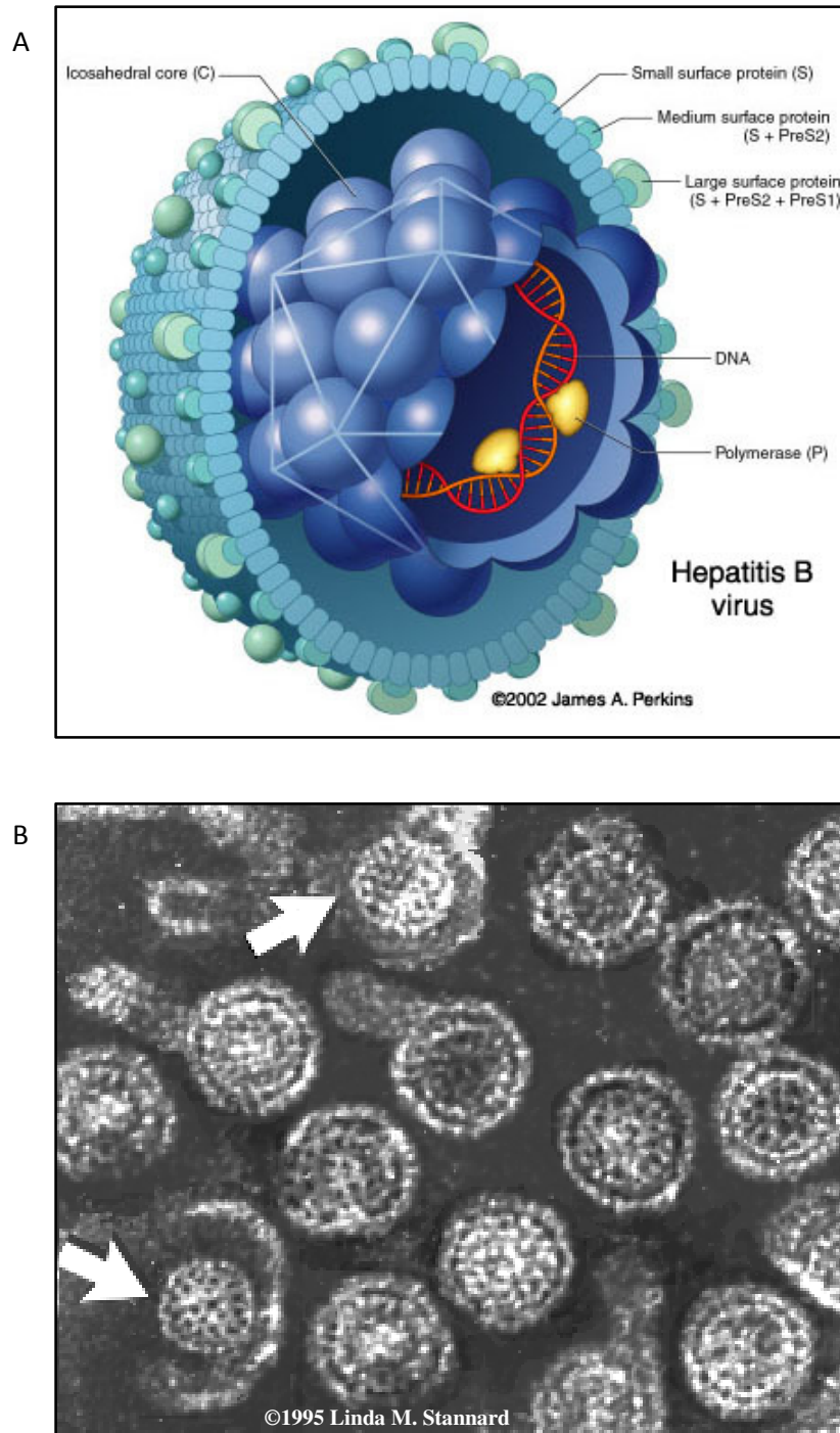
Figure 1.1: (A) Schematic representation of the HBV virion and its organization. The darker blue beads represent the core proteins of the nucleocapsid; the light blue to turquoise beads
