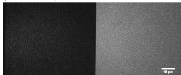
(d) Background at 638 nm taken with laser power 3/5 at 150 ms exposure time with the filter set for the FRET couple sCy3/sCy5 (see table 4.4).
