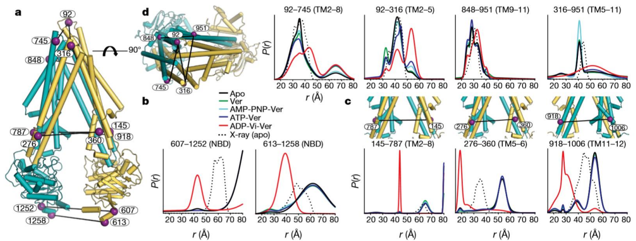
Figure 3.4: Dynamics of P-gp studied with DEER. From Verhalen et al. [2017]. (a) Several positions of P-gp are successively labelled with spins to perform DEER measurements. (b), (c), (d) Distance changes measured respectively in the NBDs, in the intracellular domains (ICDs) and in the TMDs. Conformation change is observed only upon addition of ADP-Vi-Verapamil.
