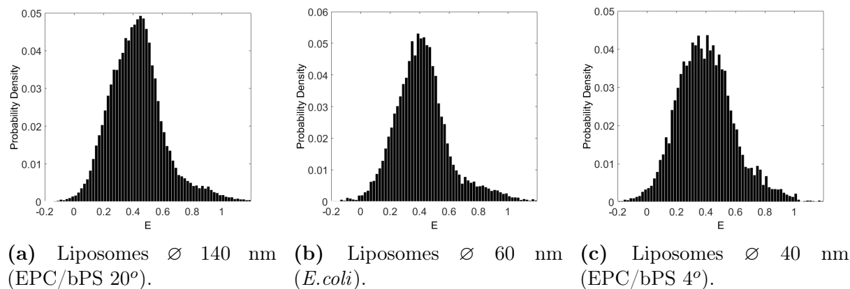
Figure 6.4: FRET distributions of Vi trapped BmrA. E distributions plotted for Vi trapped BmrA reconstituted in three different liposomes populations. Only particles exhibiting FRET signal are plotted.
