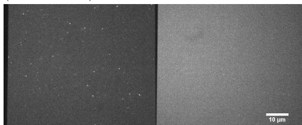
(c) Background at 532 nm taken with laser power 3/5 at 150 ms exposure time with the filter set for the FRET couple sCy3/sCy5 (see table 4.4)
