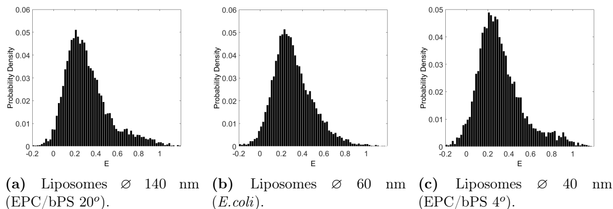
Figure 6.5: FRET distributions of ATP Vi BmrA. E distributions plotted for ATP Vi BmrA reconstituted in three different liposomes populations. Only particles exhibiting FRET signal are plotted.
