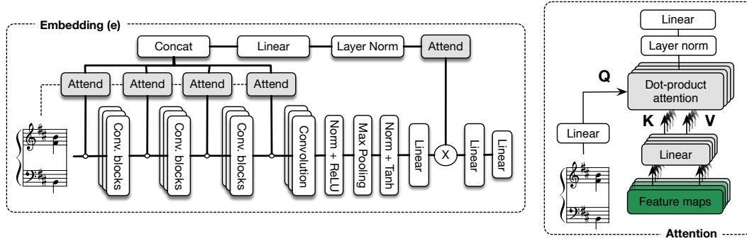
Figure 3.2: Our proposal is composed of two major parts. ( Left ) A convolutional network is augmented with a separate attention mechanism at each convolutional layer. This allows to attend the most salient information at each level of processing. ( Right ) The input acts as a query to the attention module, which works on each of the feature maps separately.
