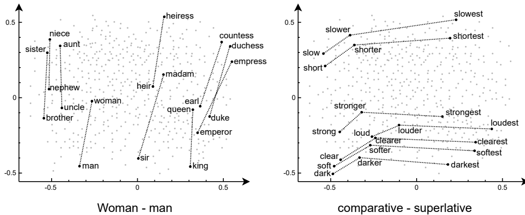
Figure 2.17: Set of visualizations that show interesting patterns relying to the vectors differences between related words in an embedding space learned with GloVe ( 'GloVe: Global Vectors for Word Representation' ).
