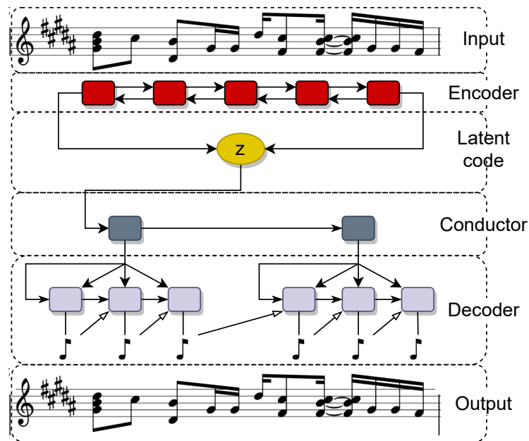
Figure 2.20: MusicVAE architecture with a hierarchical decoder. The conductor RNN provides sub-sequences from which the final output is recursively decoded by the decoder RNN (Roberts et al., 2018).
