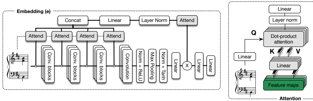
Figure 3.2: Our proposal is composed of two major parts. (Left) A convolutional network is augmented with a separate attention mechanism at each convolutional layer. This allows to attend the most salient information at each level of processing. (Right) The input acts as a query to the attention module, which works on each of the feature maps separately.
