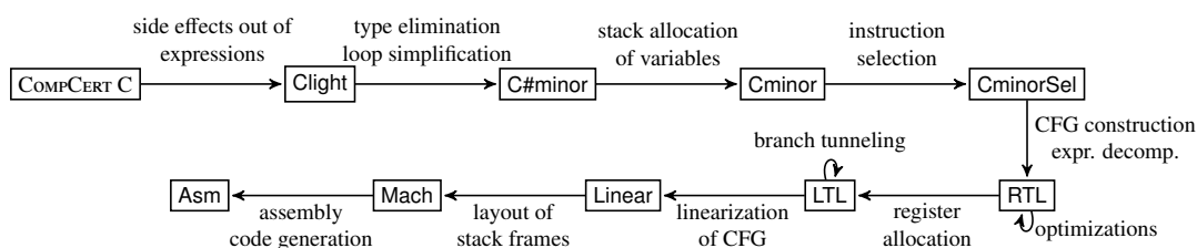
Figure 1.3.: The Intermediate Languages of COMPCERT
