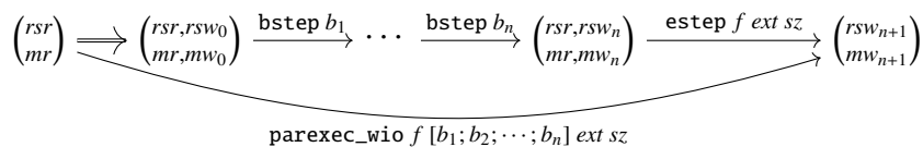
Figure 3.2.: Parallel In-Order Blockstep
