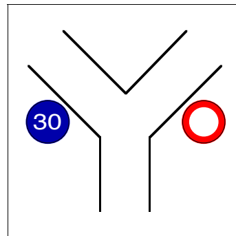
Configuration \Delta_8^A .
