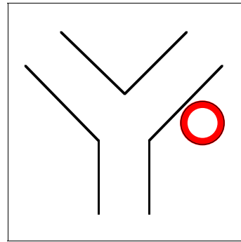
Configuration \Delta_4^A .
