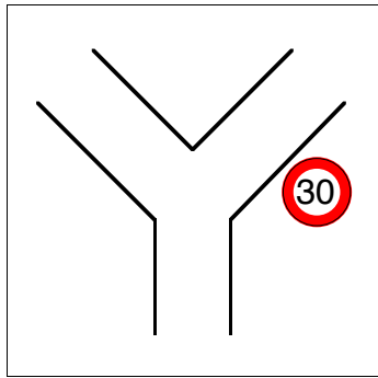
Configuration \Delta_3^A .
