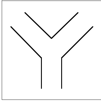
Configuration \Delta_1^A .
