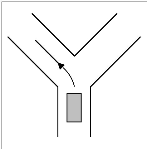
Configuration \alpha_1 .
