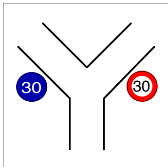
Configuration \Delta_7^A .
