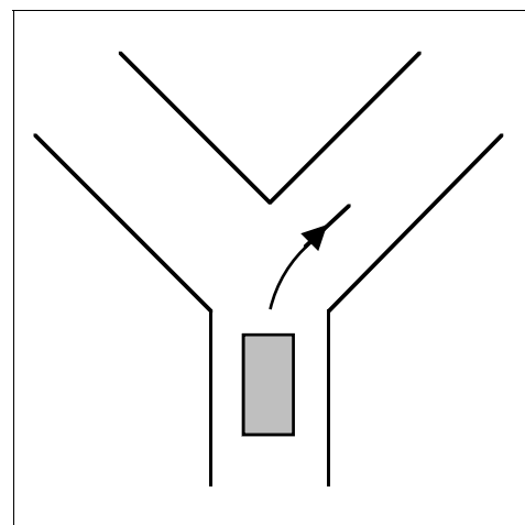
Configuration \alpha_4 .
