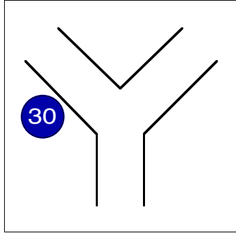
Configuration \Delta_5^A .
