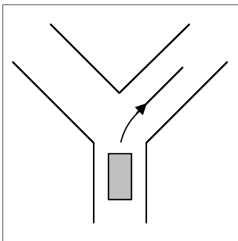
Configuration \alpha_3 .
