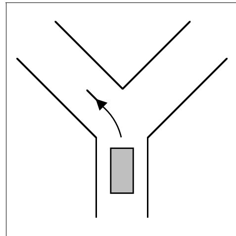
Configuration \alpha_2 .
