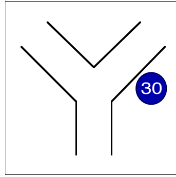
Configuration \Delta_2^A .
