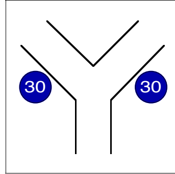
Configuration \Delta_6^A .
