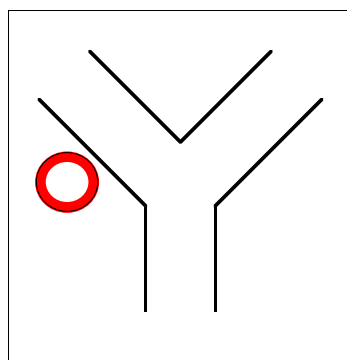
Configuration \Delta_{13}^A .
