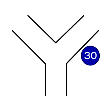
Configuration \Delta_2^A .
