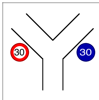
Configuration \Delta_{10}^A .
