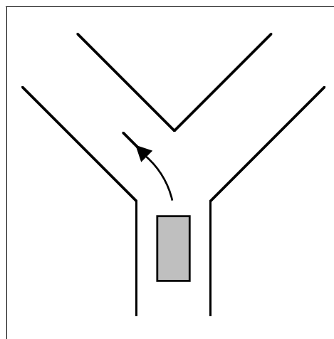
Configuration \alpha_2 .
