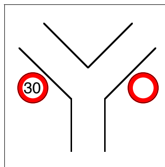
Configuration \Delta_{12}^A .
