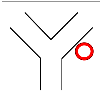
Configuration \Delta_2^A .
