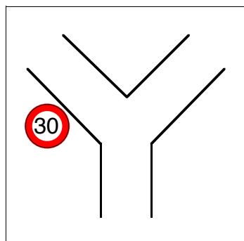
Configuration \Delta_9^A .
