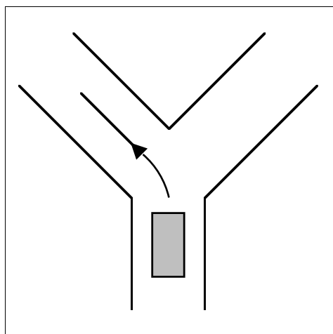
Configuration \alpha_1 .
