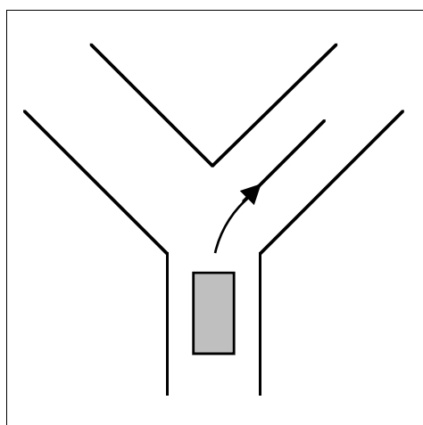
Configuration \alpha_3 .
