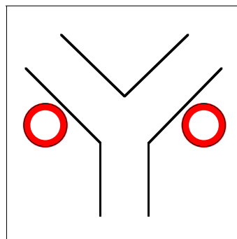
Configuration \Delta_{16}^A .
