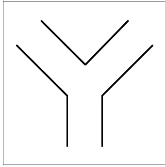
Configuration \Delta_1^A .
