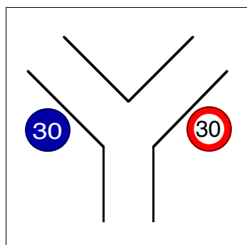
Configuration \Delta_7^A .
