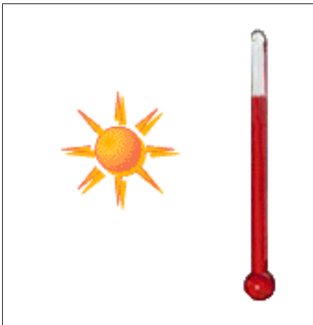
Configuration \alpha_1 .
