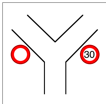
Configuration \Delta_{15}^A .
