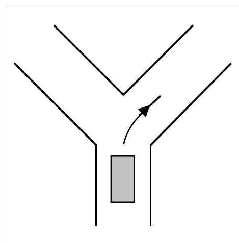
Configuration \alpha_4 .
