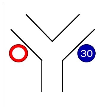
Configuration \Delta_{14}^A .
