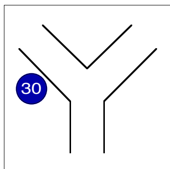
Configuration \Delta_5^A .
