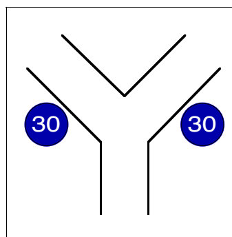
Configuration \Delta_6^A .
