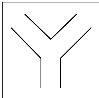
Configuration \Delta_1^A .
