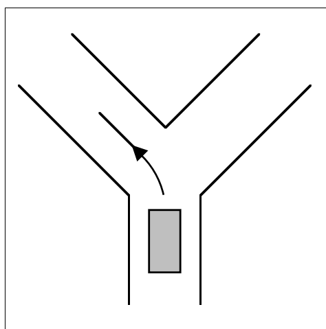
Configuration \alpha_1 .
