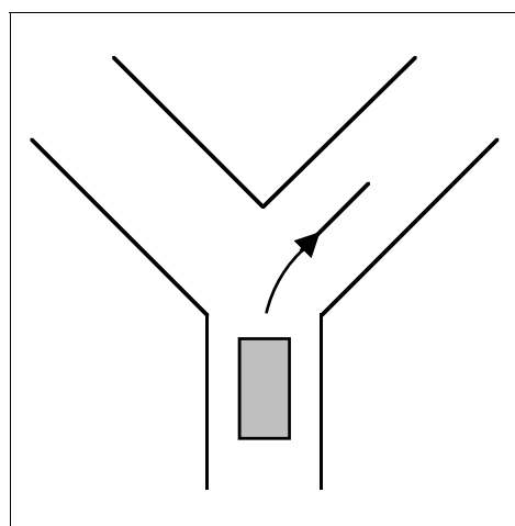
Configuration \alpha_2 .
