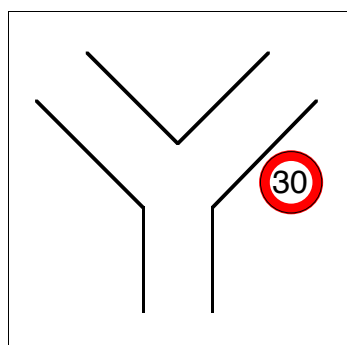
Configuration \Delta_3^A .
