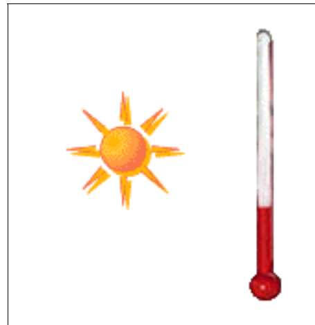
Configuration \alpha_2 .
