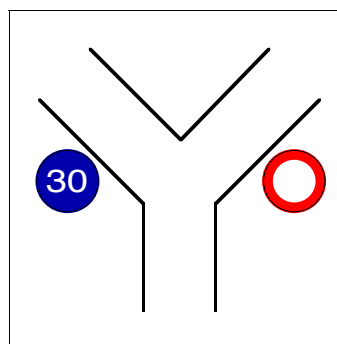
Configuration \Delta_8^A .
