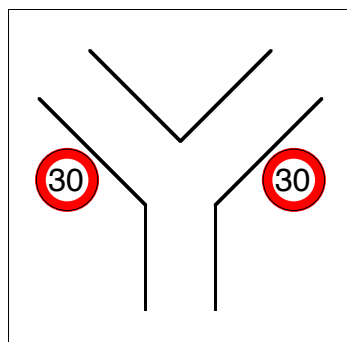
Configuration \Delta_{11}^A .
