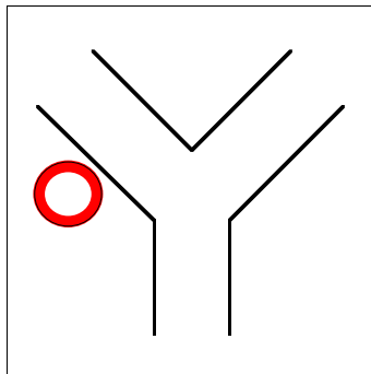
Configuration \Delta_3^A .
