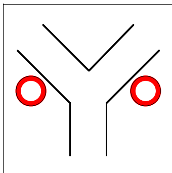
Configuration \Delta_4^A .
