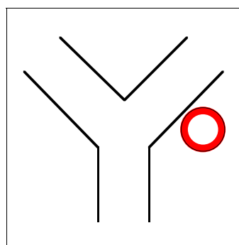
Configuration \Delta_4^A .
