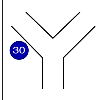
Configuration \Delta_5^A .
