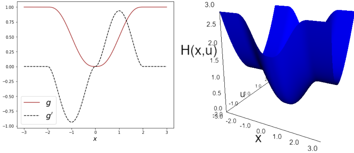
Figure 8.3 – Representation of the Hamiltonian.
