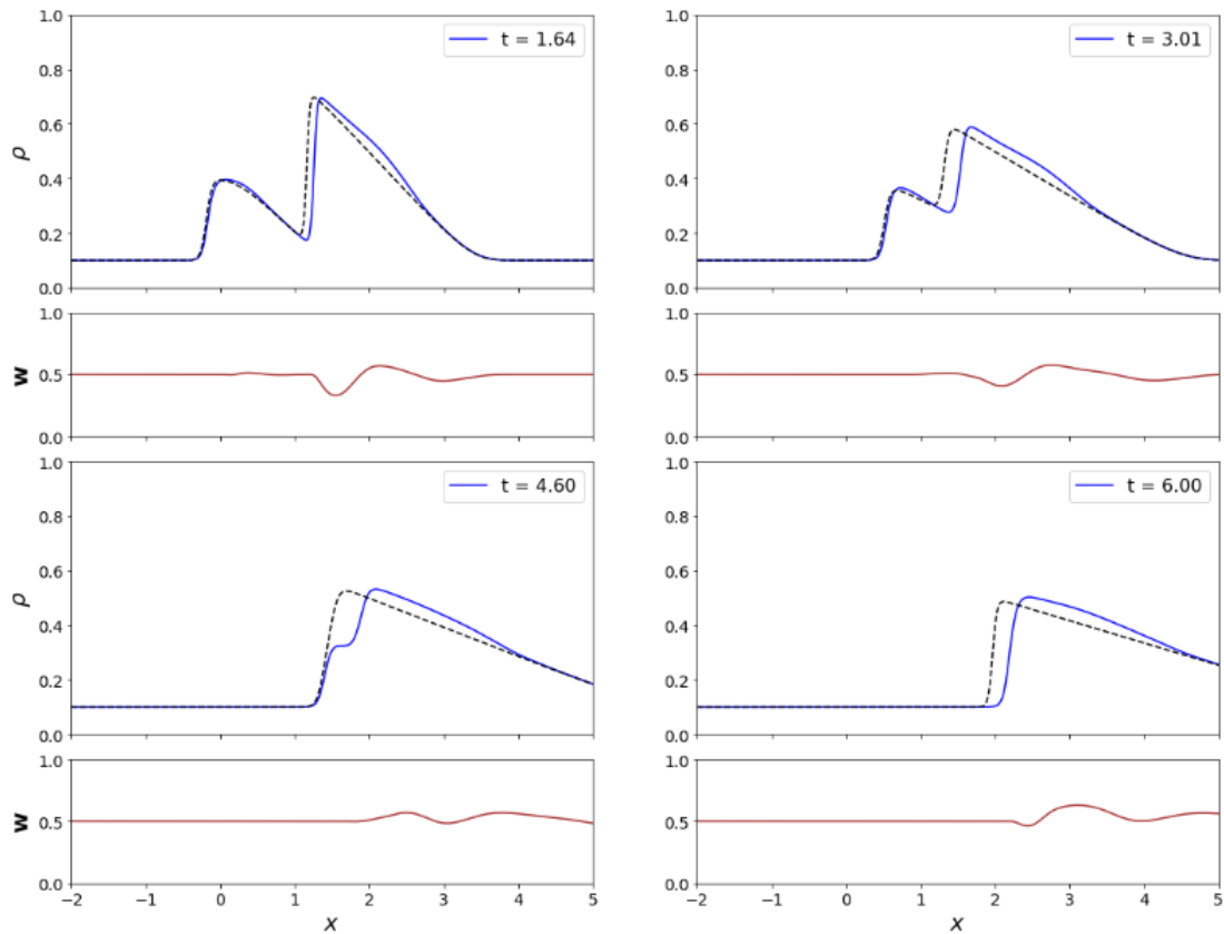
Figure 7.4 – The numerically computed solutions \rho_{\Delta}(\cdot, t), \mathbf{w}_{\Delta}(\cdot, t) at different fixed times t ; dashed lines correspond to the reference solution in absence of orderliness marker, i.e. for \omega \equiv 0 in (7.2.2); for an animated evolution of the numerical solution, follow: https://utbox.univ-tours.fr/s/AgDkkaQm9247ZEP .
