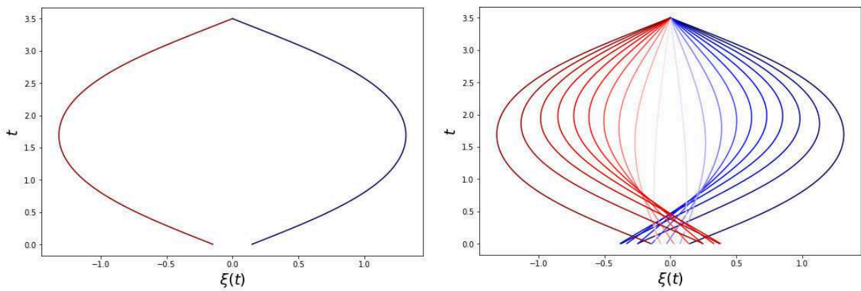
Figure 8.5 – Backward characteristics.
