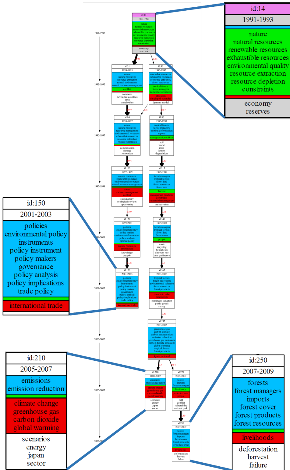
Figure 6.16: Pivot graph G^{future}(t_{14}, 0.4) over the ISTEEX corpus
