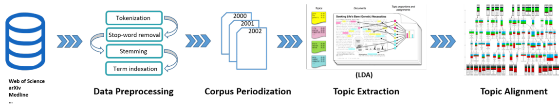
Figure 1.2: EPIQUE Workflow
