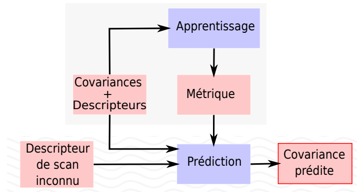
Figure 4.3.: Algorithme CELLO.
