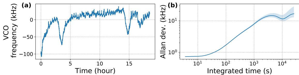
Figure 4.21: Frequency stability of the offset VCO with time series on (a) and Allan deviation on (b).
