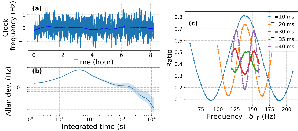
Figure 4.22: Ramsey interferometer fringes (c) centered with the hyperfine transition frequency \delta_{HF} for different interrogation time T . Time series (a) and Allan deviation (b) of the frequency stability at mid-fringe for T=40 ms. The dark blue curve on time series graph shows a moving average of 1 hour.
