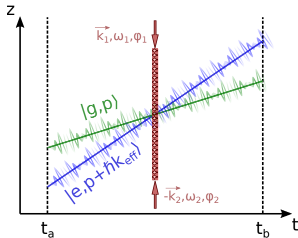
Figure 2.5: Diffracted paths when the atomic cloud is exposed to a pair of counter-propagating Raman lasers.
