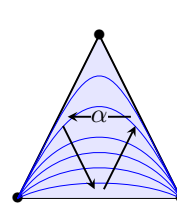
no boundary side and d(\alpha) = 1
