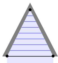
two boundary sides
