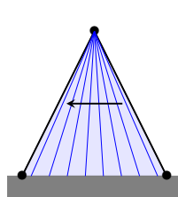
one boundary side
