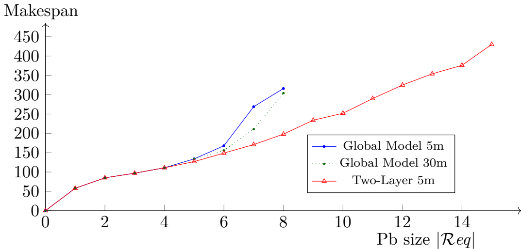
Figure 5.11: Makespan results for the Path Isolation approach.
