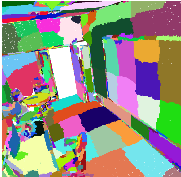
(b) Over-segmentation
