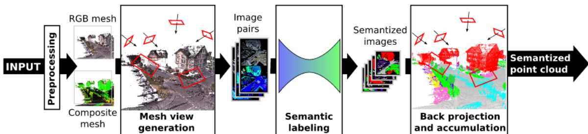
Figure 4.12: Snapnet framework for point cloud semantic segmentation. Image from [209]
