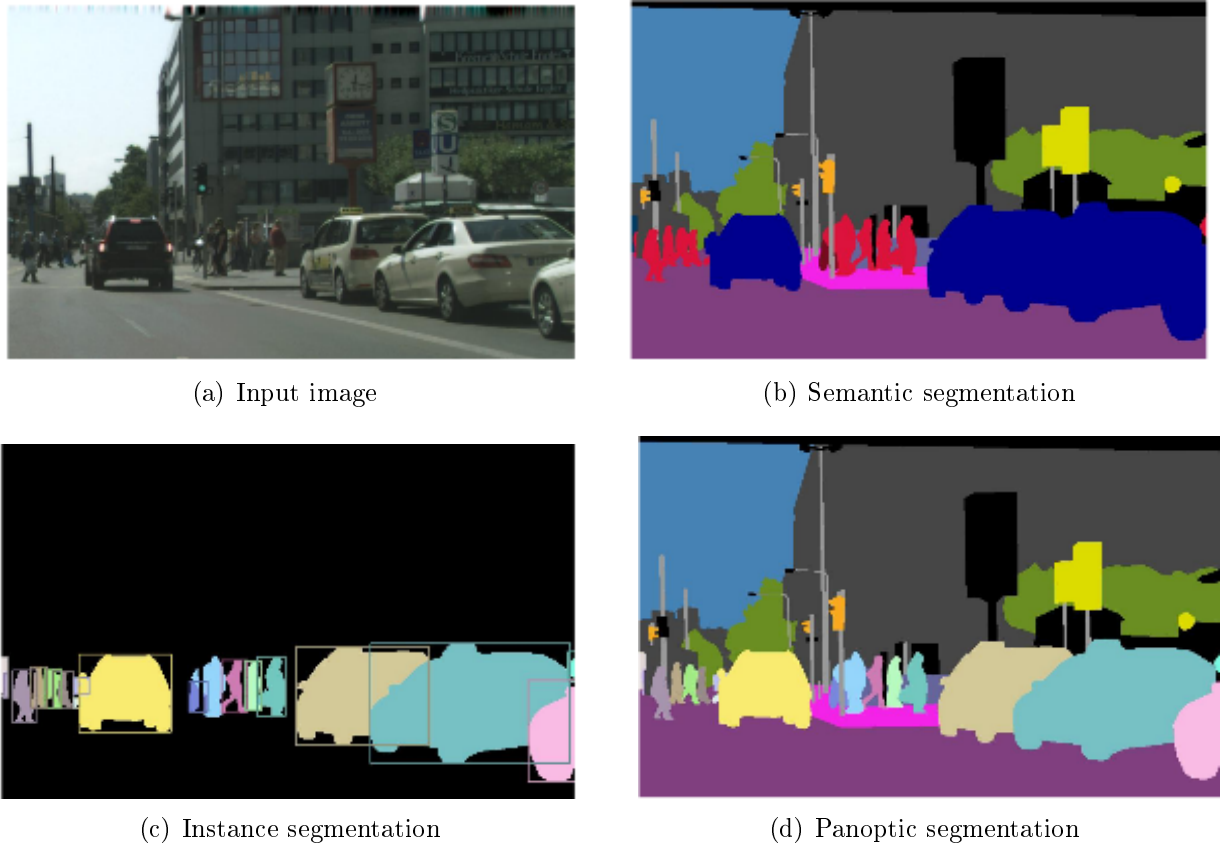
Figure 1.4: Illustration of semantic, instance and panoptic segmentation on a 2D image. Images from [6]
