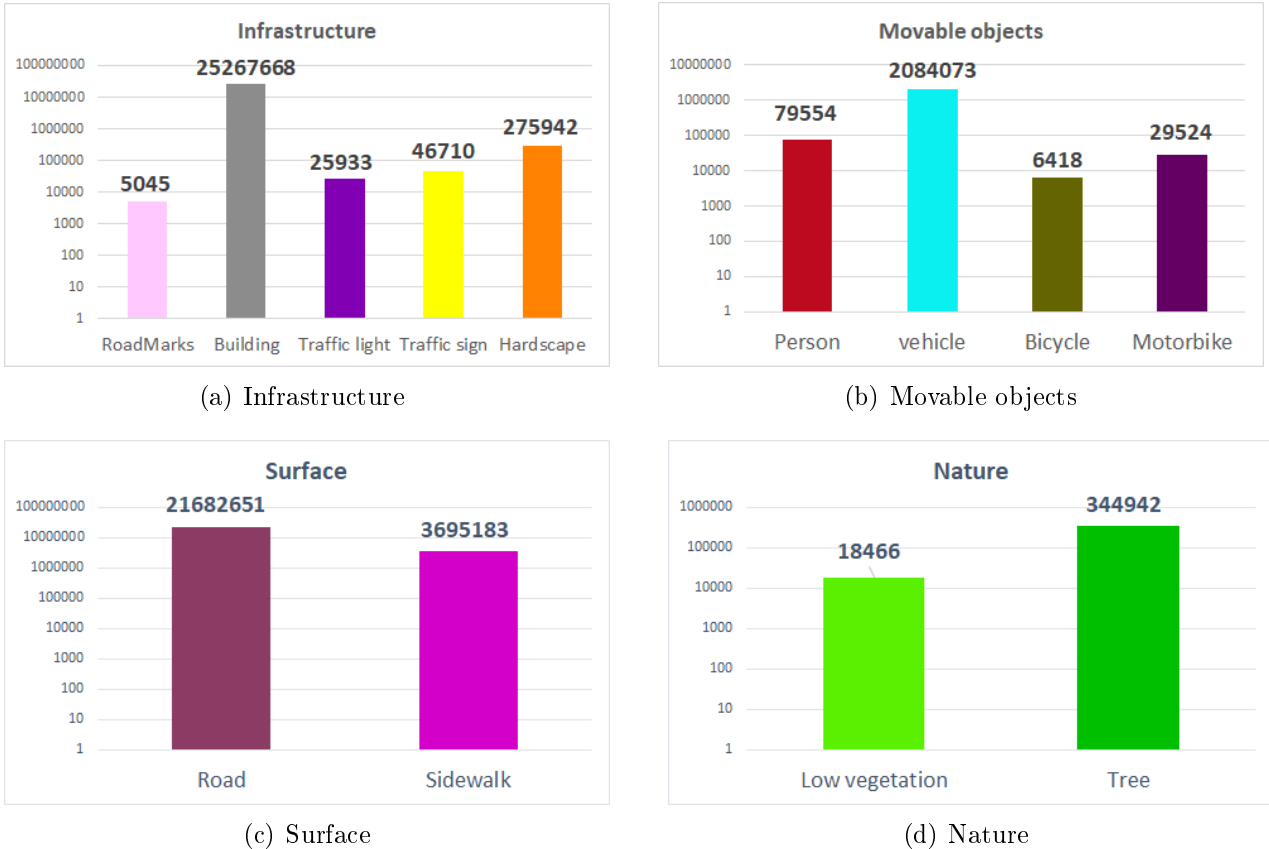
Figure 2.17: Statistics on the distribution of the annotated point clouds per-class
