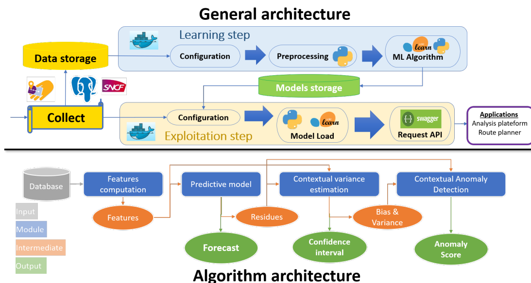
Figure 1.4.: Pipeline of IVA data analysis tool
