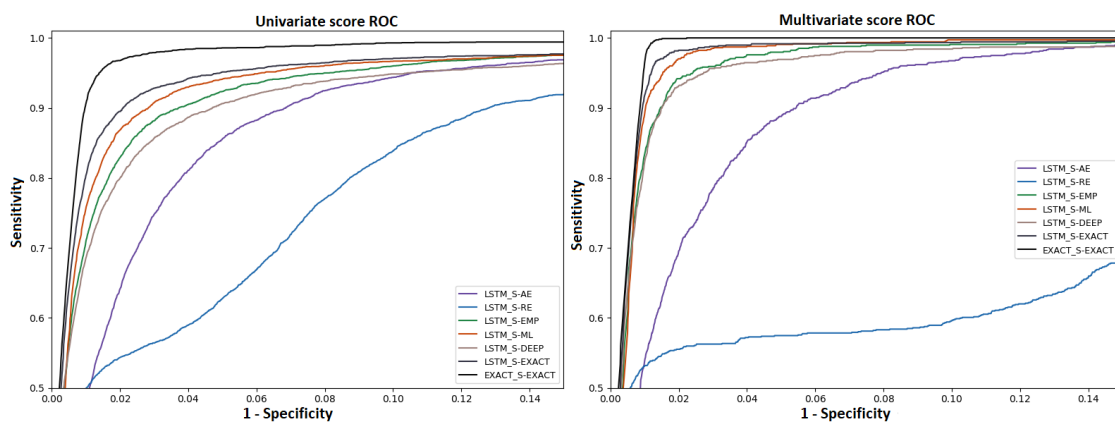
Figure 4.6.: ROC curves for the local and global scores based on the LSTM-EP residue
