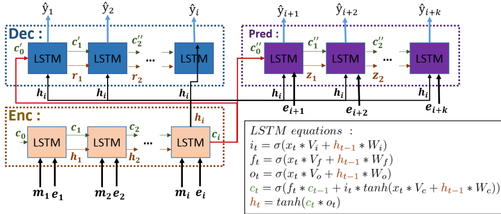
Figure 3.8.: Details of the layout of the LSTMs
