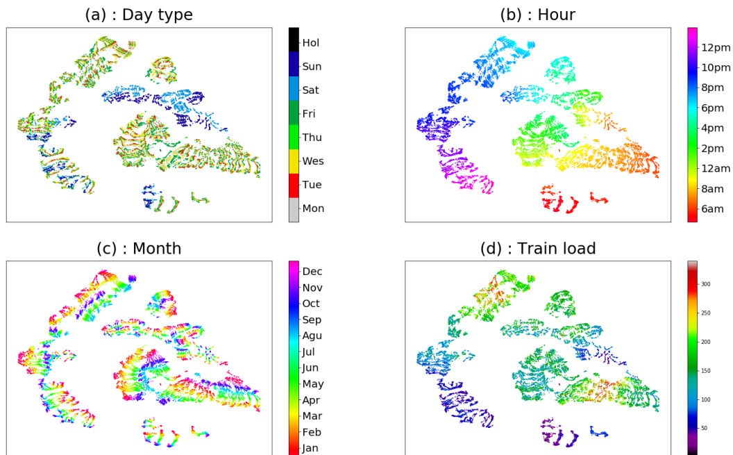
Figure 3.14.: Latent representation ( u_t ) according to contextual features with dimension reduction
