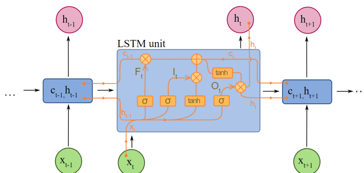
Figure 3.4.: LSTM architecture (Figure from Wikipedia, based on C. Olah 1 )
