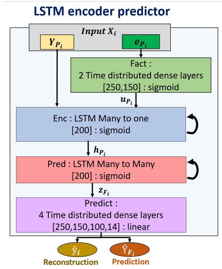
Figure 3.9.: LSTM-EP architecture with the layer size for the real data
