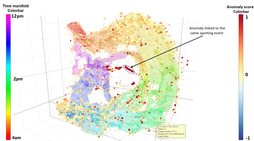
Figure 3.16.: 3D reduction of Predictive latent space ( z_t ) of suburban station with anomaly score coloration
