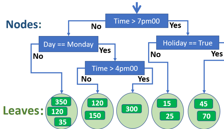
Figure 3.1.: Illustration of Decision Tree
