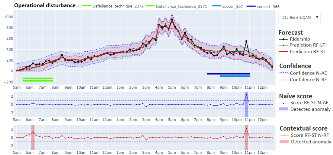
Figure 4.13.: Ridership and anomaly scores at Pie IX station on Wednesday, 5 August, 2015
