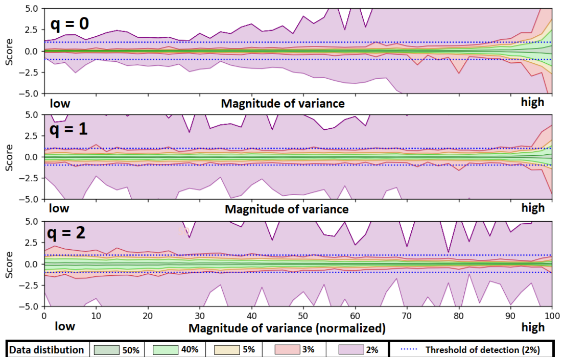
Figure 4.5.: Distribution of anomaly score (2%) as a function of variance magnitude
