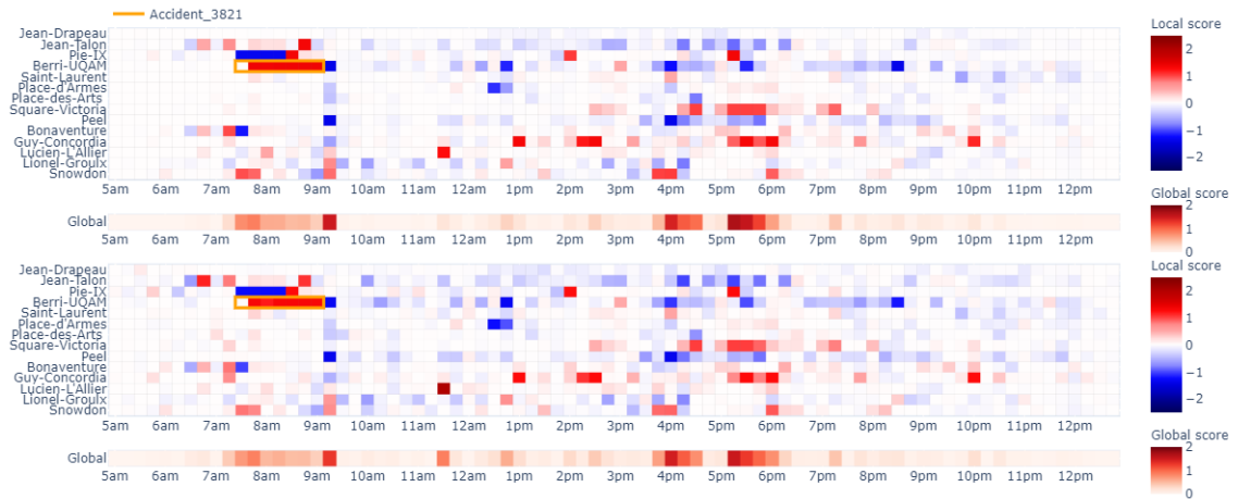
Figure 4.10.: Two anomaly scores (N-AE, N-RF) computed on Monday, 27 February, 2017
