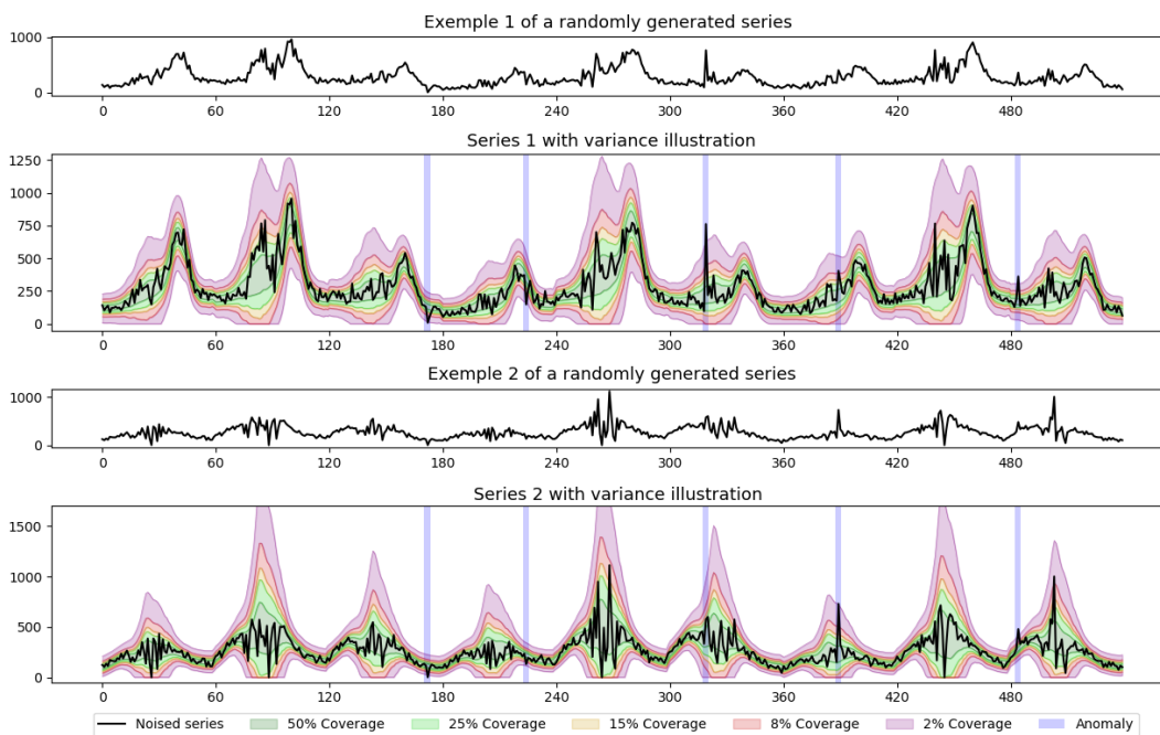
Figure 4.3.: Example of time series generated on 9 “hypothetical days”
