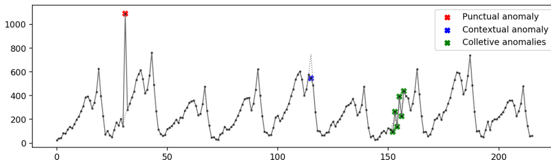
Figure 4.2.: Example of the different types of anomalies
