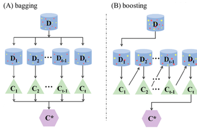
Figure 3.2.: Illustration of Bagging vs Boosting from [Yan+19]
