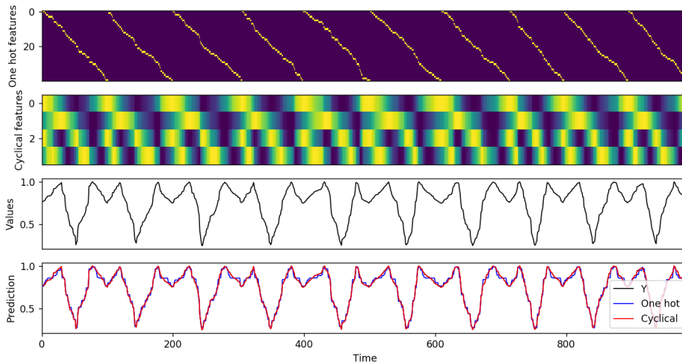
Figure 3.5.: Toy prediction using one-hot and cyclic features
