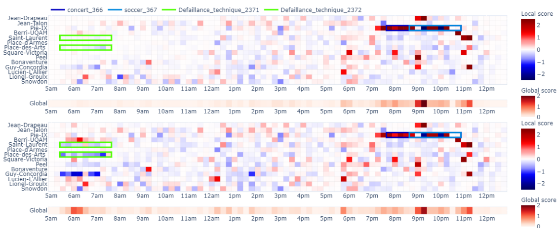
Figure 4.12.: Two anomaly scores (N-AE, NS-RF) computed on Wednesday, 5 August, 2015
