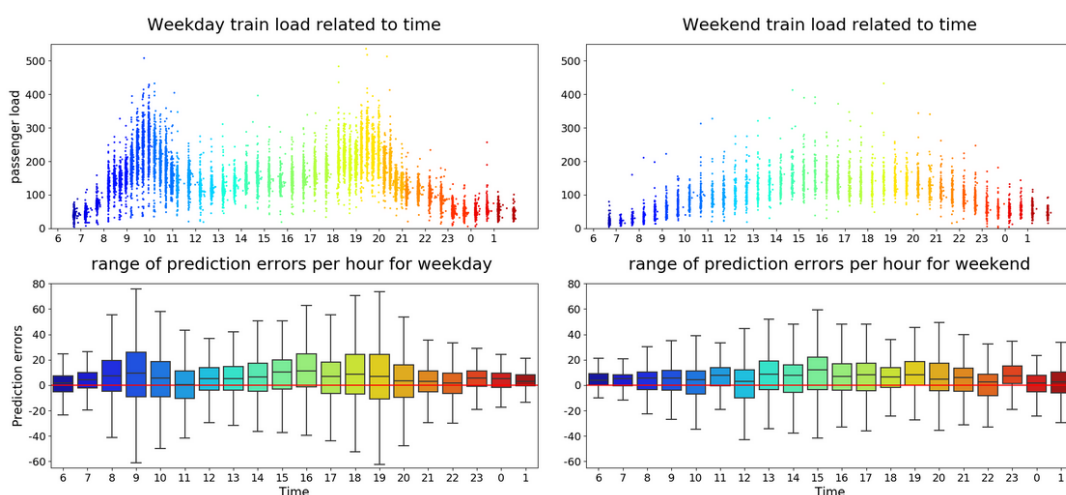
Figure 3.13.: Prediction errors depend on hour class for suburban station
