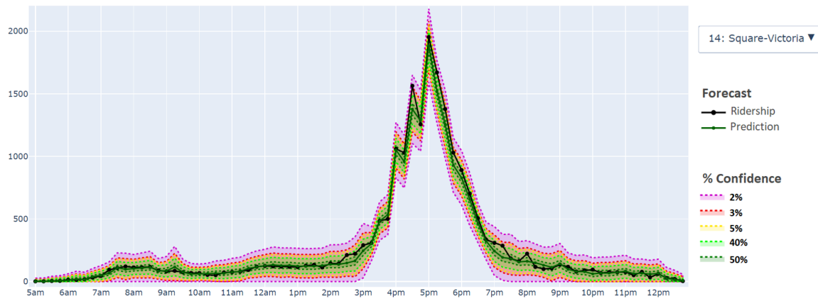
Figure 4.9.: Ridership prediction confidence at the Square Victoria station, Monday February 27
