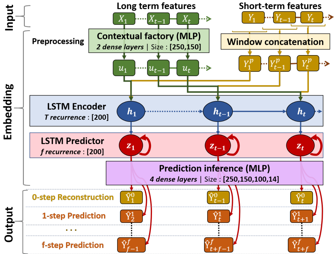
Figure A.3.: Regular LSTM-encoder predictor with underlying structured data
