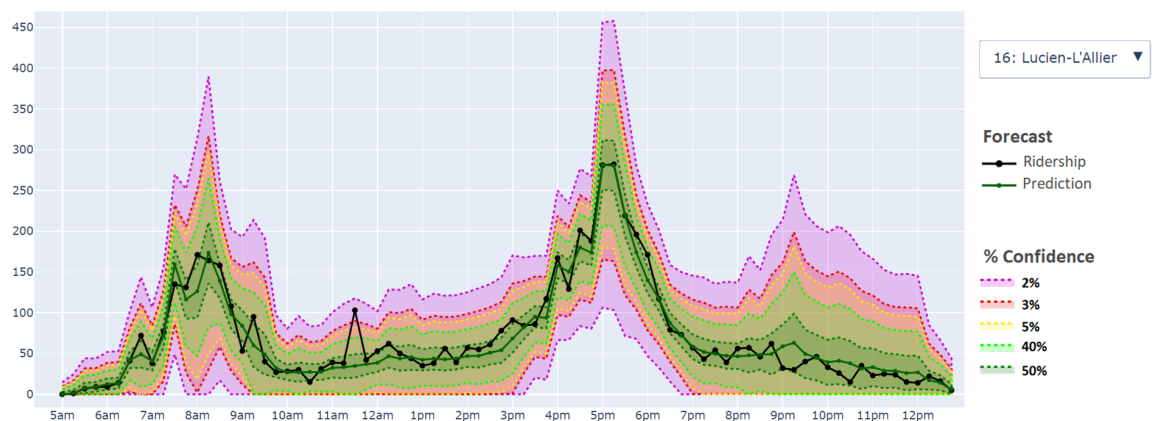
Figure 4.8.: Ridership prediction confidence at Lucien l'Allier station on Monday, February 27
