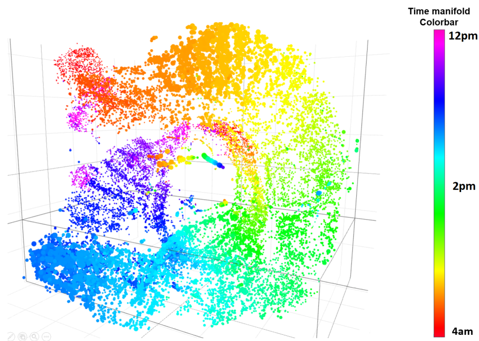
Figure 3.15.: 3D reduction of Predictive latent space ( z_t ) of suburban station with time coloration
