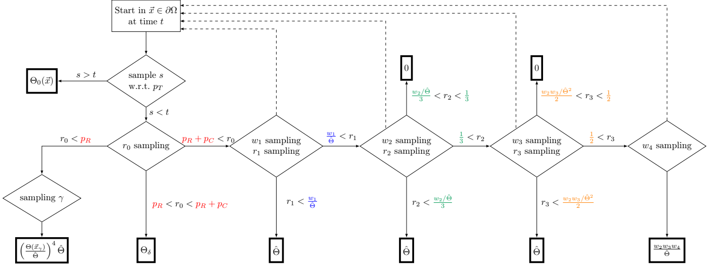
Figure 1. Branching Algorithm
