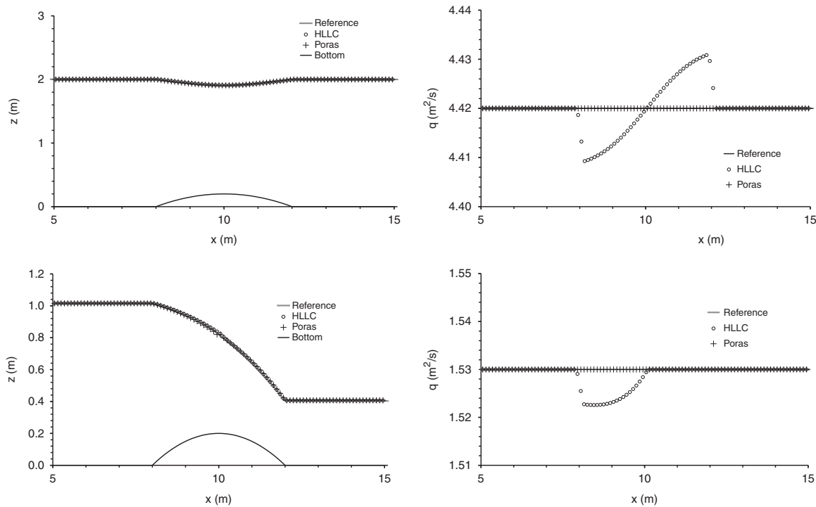
Figure 11. One-dimensional flow over a bump ( T_{2,(sub,trans)} ). Reference, HLLC and PorAS solutions; Left, simulated water level; Right, simulated unit discharge; Top, subcritical test case; Bottom, transcritical test case.
