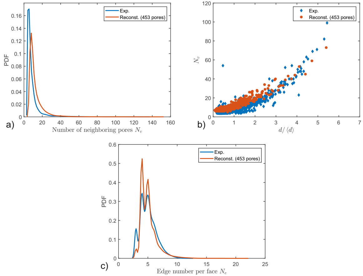
Figure III.17: Comparison of foam morphology between the experimental results and the data estimated on the numerical model, for (a) the number of neighbor, (b) the correlation between the number of neighbors and the normalized equivalent diameter, and (c) the number of edges per face.
