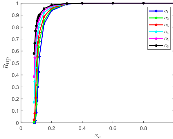
Figure IV.20: Open density R_{\text{op}} as a function open membrane proportion x_o .
