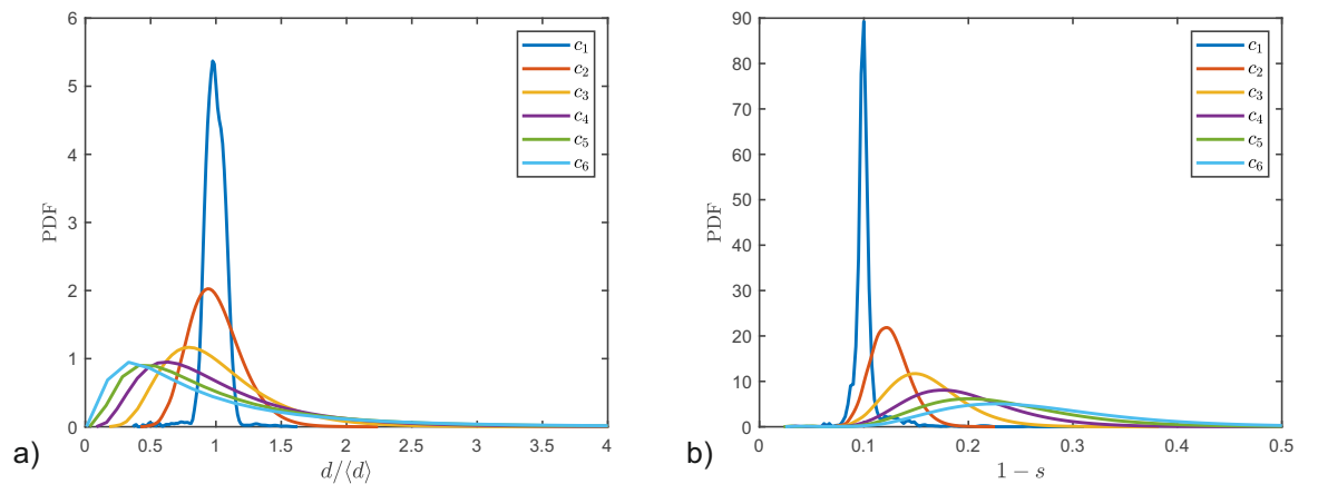
Figure IV.5: Distribution of a) Normalized pore size d/\langle d \rangle and b) 1 - \text{Sphericity} for generated random foams.
