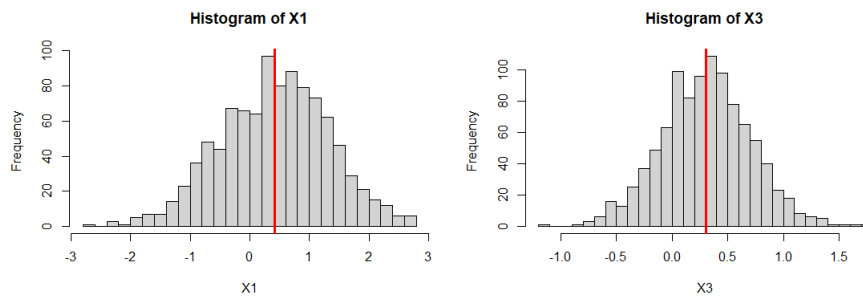
FIGURE 3.8: Histogram for observations of X_1 and X_3 .
