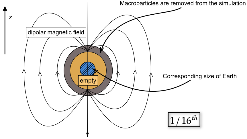
Figure 5.3: Sketch of the obstacle in LatHyS. Magnetic field lines are represented with curved arrows, starting from just the outside of the yellow circle. The obstacle is represented in grey and yellow. The comparative size of Earth is represented in blue.
