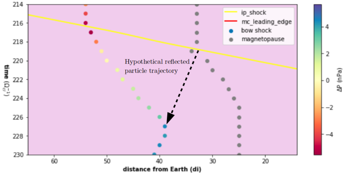
Figure 6.21: Zoom on figure 6.16: Temporal evolution of the positions along the Sun-Earth line of the bow shock (multicolored dots) and magnetopause (grey dots), as they are impacted by the arrival of the interplanetary shock (gold line). A dashed black arrow has been added to mark the hypothetical trajectory of particle that would be reflected at the magnetopause and reach back the bow shock to participate in its expansion.
