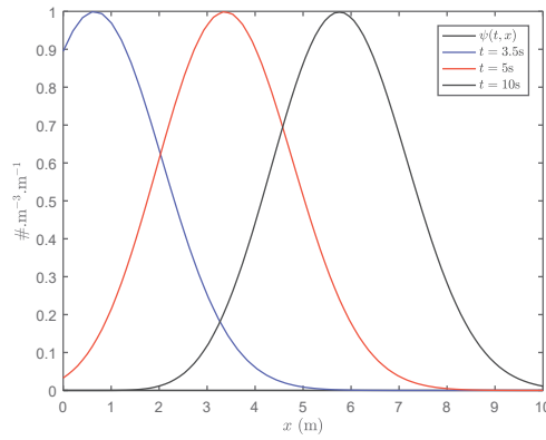
(c) Simulation of the PSD \psi .
