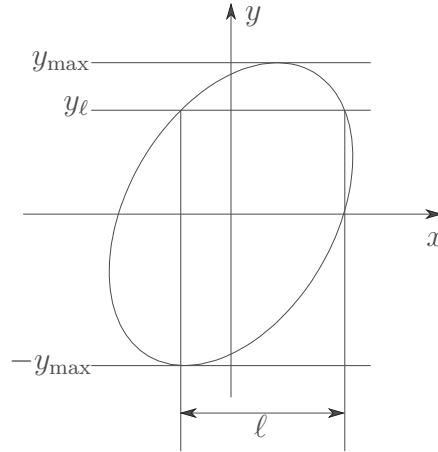
Figure 7.3 – Length \ell of a horizontal chord on an ellipse at y = y_\ell \in [-y_{\max}, y_{\max}] .
