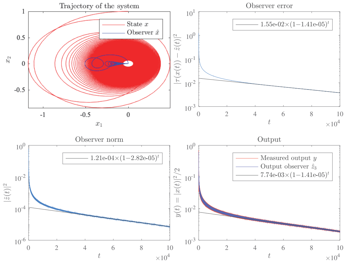
Figure 4.2 – Numerical simulation of system (4.12) with parameters given in Table 4.1. The map \tau is the embedding defined by (4.5) ( Top left ) The trajectory (x, \hat{x}) of the system seems to converge to the origin. ( Top right ) The observer error is non-increasing, as stated by (4.9), but the convergence to 0 is slow. A linear regression indicates an exponential rate about -1.41 \times 10^{-5} . ( Bottom left ) The observer tends towards the origin with exponential rate about -2.82 \times 10^{-5} . At t = 10^5 , the observer squared norm is about 10^{-5} . ( Bottom right ) The output, which is half the square of the state norm, has the same convergence rate as the observer. At t = 10^5 , the state squared norm is about 10^{-3} .
