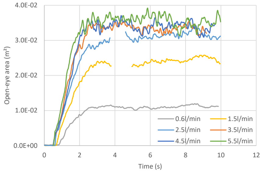
Figure 4.22: Time evolution of the open-eye area for different air flow rates with a minimum grid size of \Delta x = 527 \mu\text{m} .
