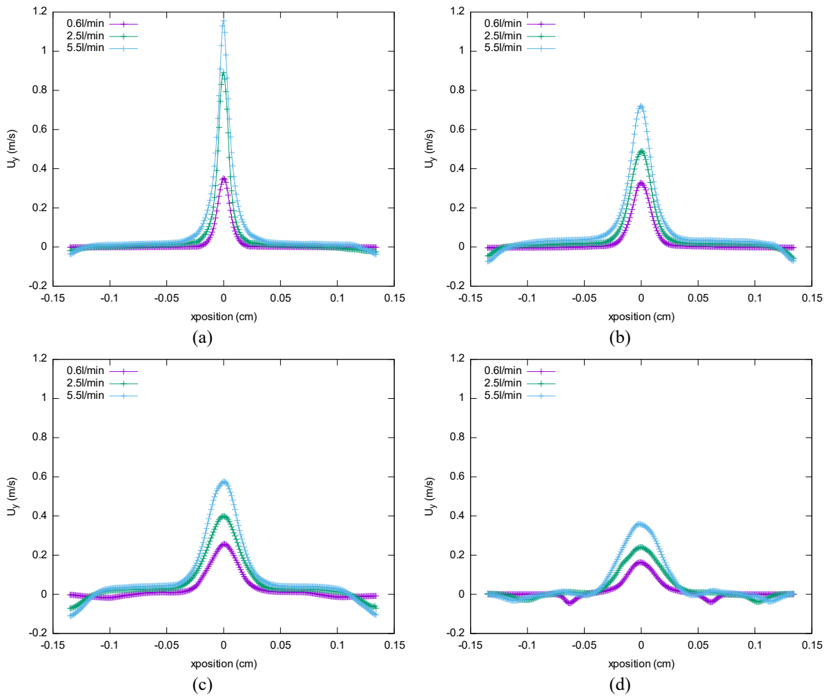
Figure 4.28: Time-averaged vertical velocity along the horizontal position for different air flow rates and with a minimum grid size of \Delta x = 527 \mu\text{m} . The interpolation is done along different lines at a given vertical position. a): y = 0.05\text{cm} ; b): y = 0.1\text{cm} ; c): y = 0.15\text{cm} ; d): y = 0.2\text{cm} .
