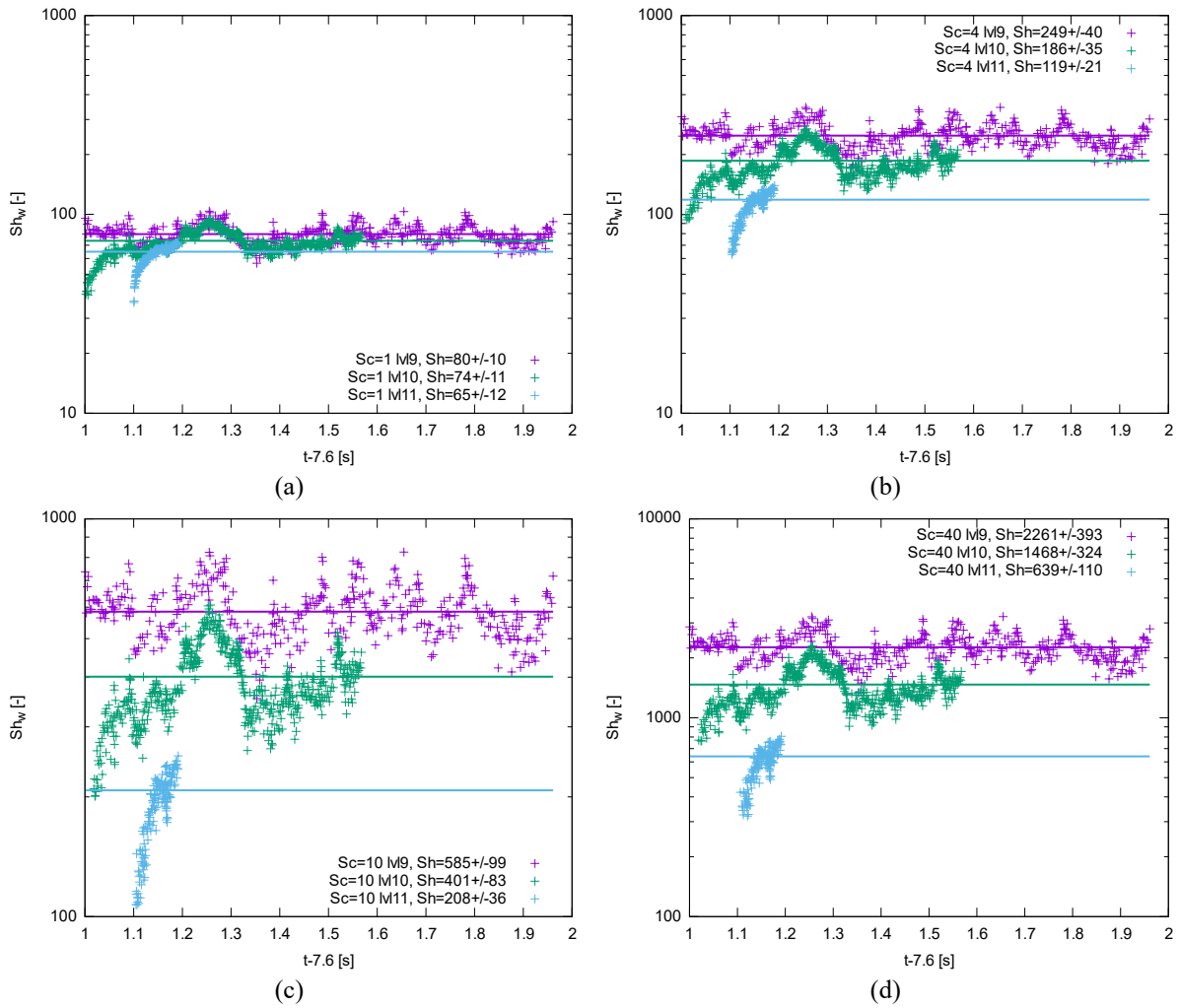
Figure 11.3: Time evolution of the Sherwood number in water with different mesh resolution at a fixed air flow rate of Q = 3.5\text{l/min} . (a) Sc_w = 1 ; (b) Sc_w = 4 ; (c) Sc_w = 10 ; (d) Sc_w = 40 .
