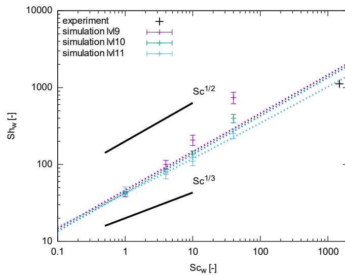
Figure 8.24: Fit of the numerical Sherwood number in water with standard deviation as a function of the Schmidt number at an air flow rate Q = 0.6 l/min and for different maximum numbers of cells in one direction. The black cross represents our experimental result.
