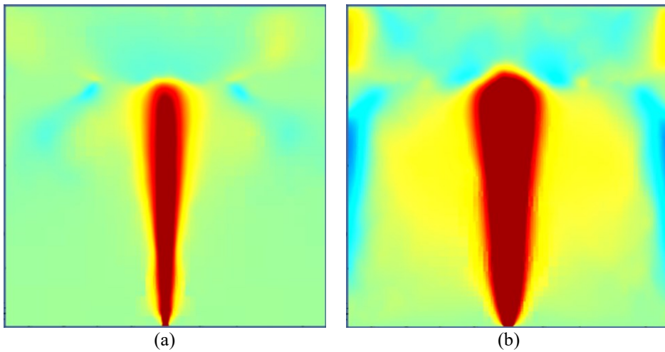
Figure 4.26: Time-averaged vertical velocity in a slice in the middle of the domain. The results are obtained with a minimum grid size of \Delta x = 527 \mu\text{m} . Maximum and minimum value are represented respectively with red and blue colours. a): Q = 0.6\text{l/min} ; b): Q = 5.5\text{l/min} .
