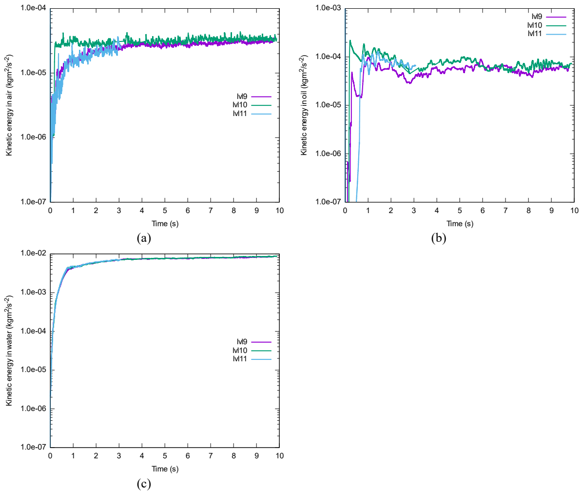
Figure 4.13: Comparison of the phase-specific Kinetic energy obtained at the same air flow rate of Q = 0.6\text{l}/\text{min} with different mesh resolutions. a): Kinetic energy of the air phase; b): Kinetic energy of the oil phase; c): Kinetic energy of the water phase
