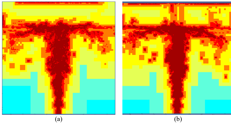
Figure 4.10: Front view of the simulation where we display the maximum mesh resolution in one direction at the same air flow rate Q = 0.6\text{l}/\text{min} . The minimum and maximum values are coloured respectively with blue and red colour. a): minimum grid size of \Delta x = 527 \mu\text{m} at t = 8.1\text{s} ; b): minimum grid size of \Delta x = 264 \mu\text{m} at t = 8.1\text{s} .
