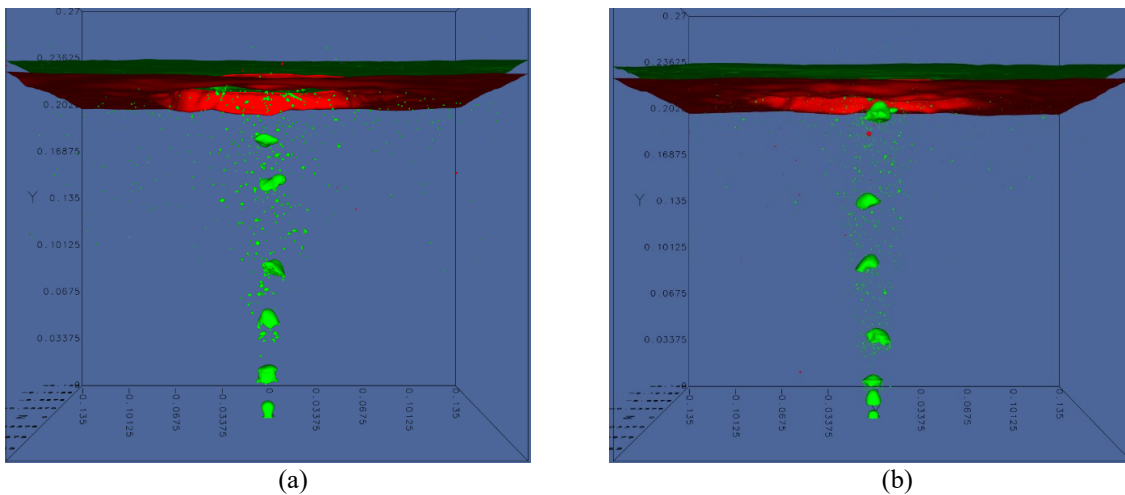
Figure 4.11: Front view of the simulation where we display instantaneous air and oil interfaces coloured respectively in green and red obtained at the same air flow rate Q = 0.6\text{l}/\text{min} . a): minimum grid size of \Delta x = 527 \mu\text{m} at t = 8.1\text{s} ; b): minimum grid size of \Delta x = 264 \mu\text{m} at t = 8.1\text{s} .
