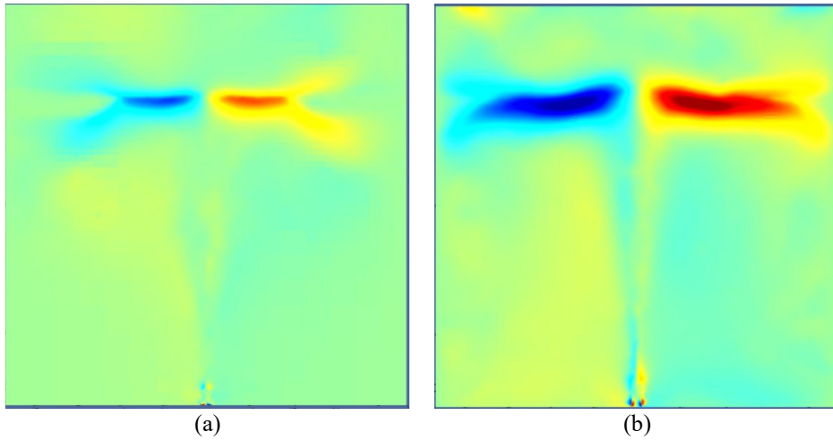
Figure 4.25: Time-averaged horizontal velocity in a slice in the middle of the domain. The results are obtained with a minimum grid size of \Delta x = 527 \mu\text{m} . Maximum and minimum value are represented respectively with red and blue colours. a): Q = 0.6\text{l/min} ; b): Q = 5.5\text{l/min} .
