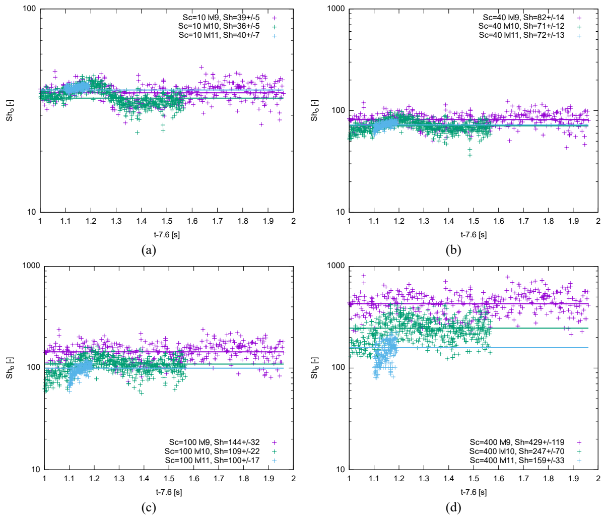
Figure 11.4: Time evolution of the Sherwood number in oil with different mesh resolution at a fixed air flow rate of Q = 3.5 l/min. (a) Sc_o = 10 ; (b) Sc_o = 40 ; (c) Sc_o = 100 ; (d) Sc_o = 400 .
