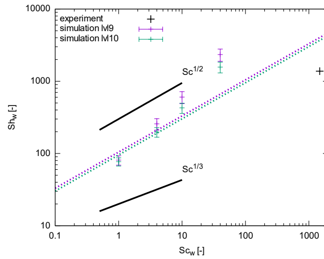
Figure 11.9: Fit of the numerical Sherwood number in water with standard deviation in function of the Schmidt number at an air flow rate Q = 4.5 l/min and for different maximum number of cells in one direction. The black cross represents our experimental result.
