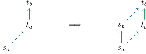
Figure 4.2: Axiom condition
