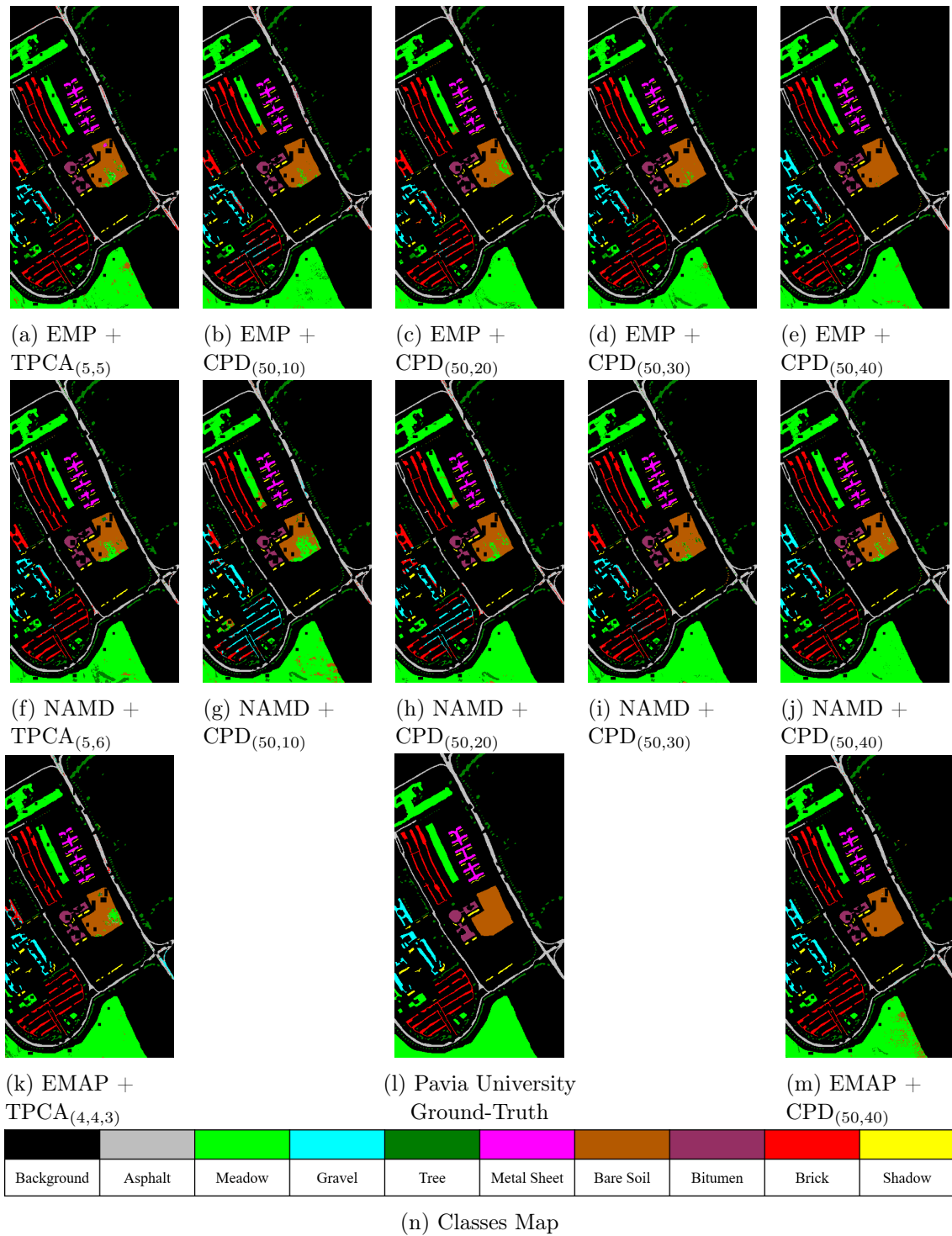
Figure 4.10: Classification maps for Pavia University HSI.
