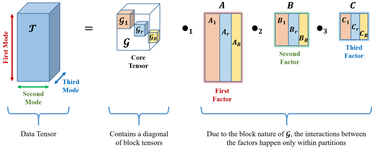
Figure 2.10: Illustration of the elements of a third-order BTM in general Tucker form.
