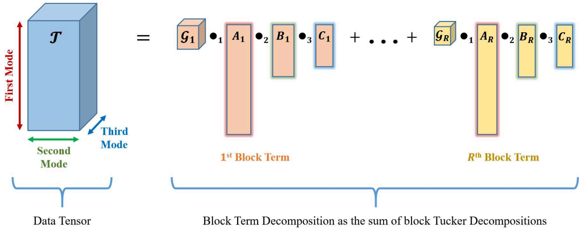
Figure 2.11: Illustration of a third-order BTM as the sum of block Tucker Decompositions.
