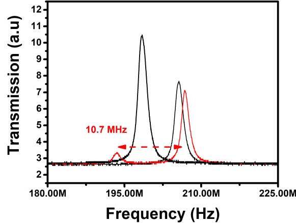
Figure 3.5: Mode-hopping of non-resonant Brillouin laser cavity, observed through a Fabry-Perot analyzer in different time intervals (black signal). Red signal shows that we can observe two resonant modes at the same time under the gain bandwidth.
