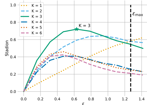
Fig. 5.12.: Stadion paths on the 4clusters_corner data set. K = 3 is selected although K^* = 4 .
