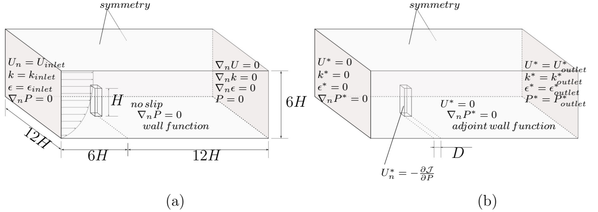
Figure 3.1 – Settings and boundary conditions of flow solution (a) and adjoint solution (b). A revoir les polices qui se chevauchent.
