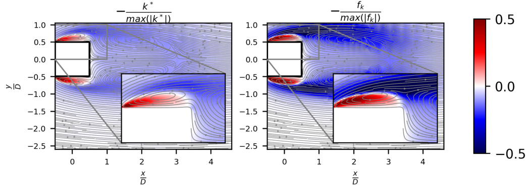
Figure 6.2 – Adjoint turbulence kinetic and the constrained control at horizontal plane with normalized height z/D = 3.33 . Variables are normalized by their in-plan peak values.
