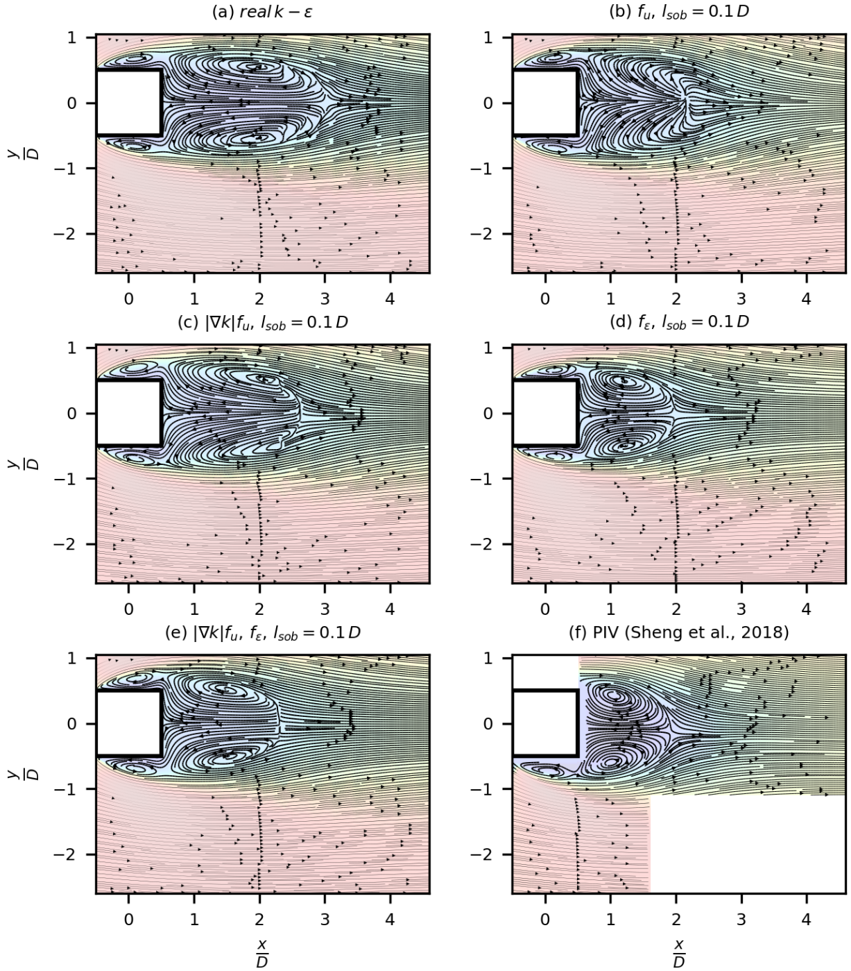
Figure 6.23 – Flow topology (2D) on horizontal plane at normalized height z/D = 3.33 . Comparison with flow reconstruction, (e), under a correction of a structured force with a modified closure applied on \epsilon budget with no penalization, (b), raw-force, (c), structured force, with default closure, and (d), modified closure made at the \epsilon budget. The steepest descent direction is improved for all algorithms by the use of Sobolev gradient with filtering length scale l_{sob} = 0.1D .
