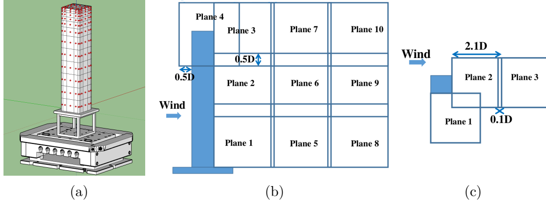
Figure 2.2 – Measurement configuration: (a), Pressure traps configuration; (b), Vertical PIV planes; (c), Horizontal PIV planes at normalized 4 heights; z/H_{ref} = 1 ( z/D = 3.33 ), z/H_{ref} = 0.75 ( z/D = 2.5 ), z/H_{ref} = 0.38 ( z/D = 1.26 ), z/H_{ref} = 0.19 ( z/D = 0.63 ).
