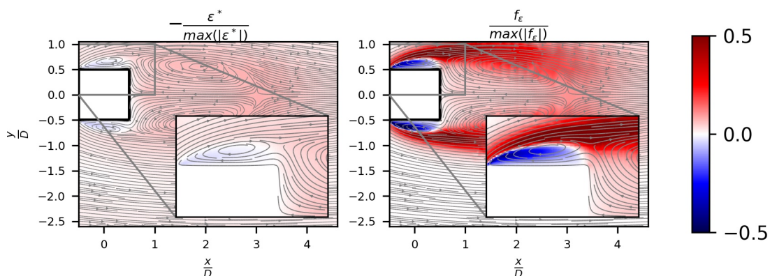
Figure 6.6 – Adjoint turbulence dissipation and the constrained control at horizontal plane with normalised height z/D = 3.33 . Variables are normalised by their in-plan peak values.
