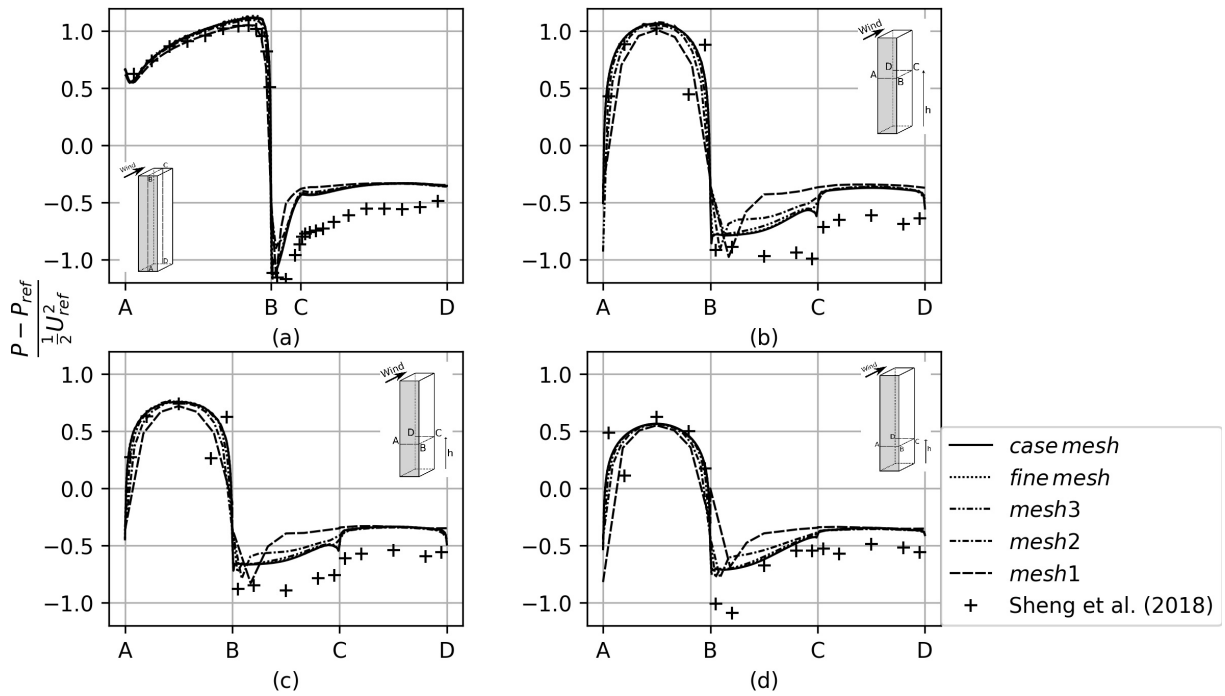
Figure 2.11 – Effects of near-structure mesh refinement on the mean pressure coefficients along the building facades.
