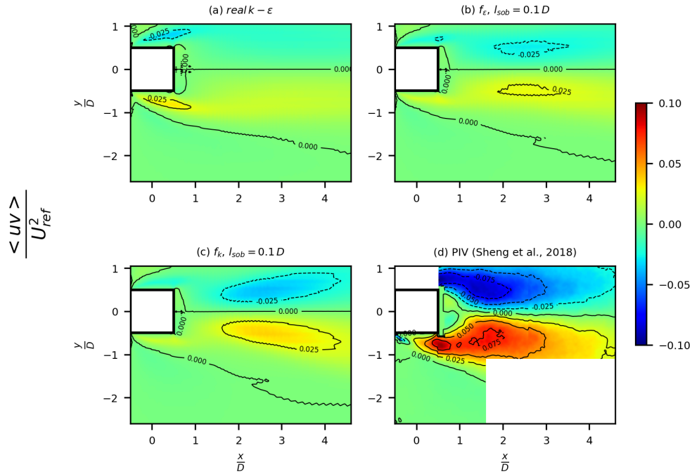
Figure 6.15 – 2D contours of Reynolds stress component \langle uv \rangle on horizontal plane at normalized height z/D = 0.63 with local constraint correction. Comparison is made between a direct k budget correction and \epsilon budget correction.
