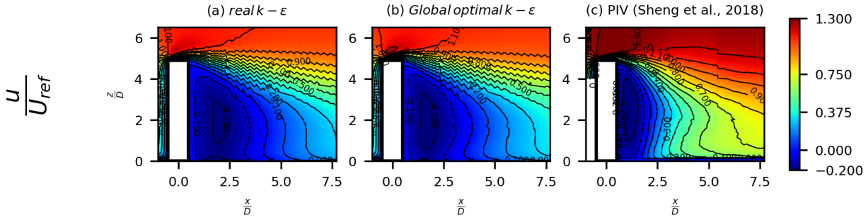
Figure 4.12 – Comparison of mean stream-wise contour between CFD (scenario B ) and Re. Sheng (PIV) experiments at symmetry plane with normalised height \frac{z}{H_{ref}} = 1 .
