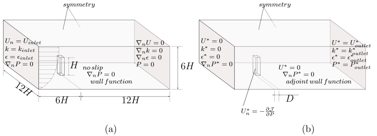
Figure 3.1 – Settings and boundary conditions of flow solution (a) and adjoint solution (b). A reservoir les poches qui se chevauchent.
