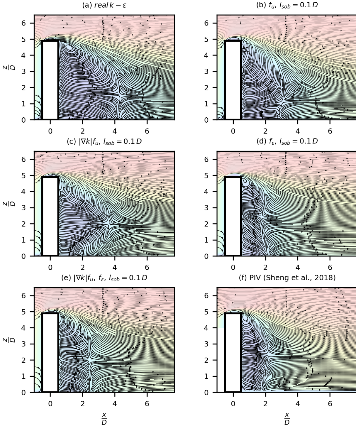
Figure 6.22 – Flow topology (2D) on symmetry plane. Comparison with flow reconstruction, (e), under a correction of a structured force with a modified closure applied on \epsilon budget with no penalization, (b), raw-force, (c), structured force, with default closure, and (d), modified closure made at the \epsilon budget. The steepest descent direction is improved for all algorithms by the use of Sobolev gradient with filtering length scale l_{sob} = 0.1 D .
