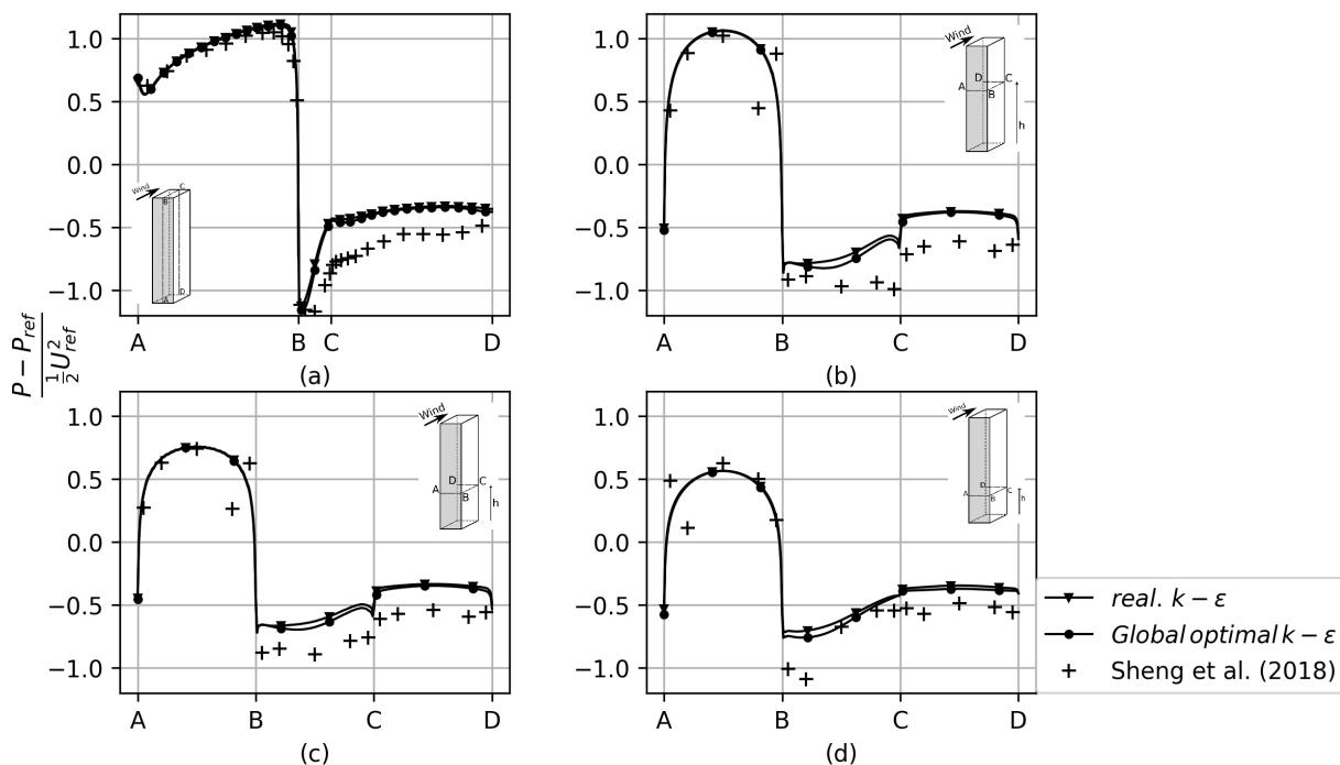
Figure 4.9 – Comparison of pressure coefficient profiles between CFD (scenario B ) and experimental results along building facades. Contours are taken at building symmetry plan, (a) and three horizontal plans at z/H_{ref} = 1 , (b), z/H_{ref} = 0.27 , (c) and z/H_{ref} = 0.19 , (d), respectively.
