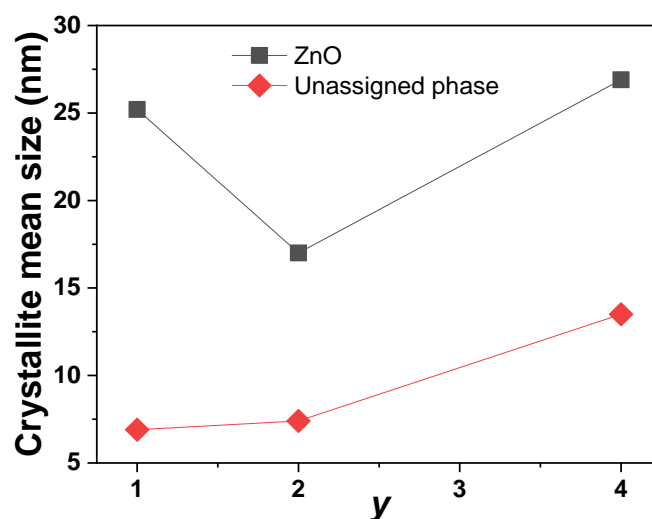
Figure 4.10 Diffraction domain size of ZnO (squares) and the unassigned phase (diamonds) of three silica-coated samples ( 3.8\text{Si-}y\text{A} ( y = 1, 2, \text{ and } 4 )) in function of the amount of \text{NH}_4\text{OH} in solution A. The size of the unassigned phase is estimated by Scherrer equation from the peak at 2\theta = 33.4^\circ .
