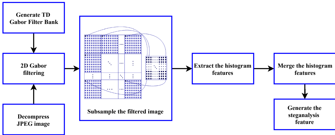
FIGURE 3.11: GFR feature extraction process [Song et al. , 2015]
