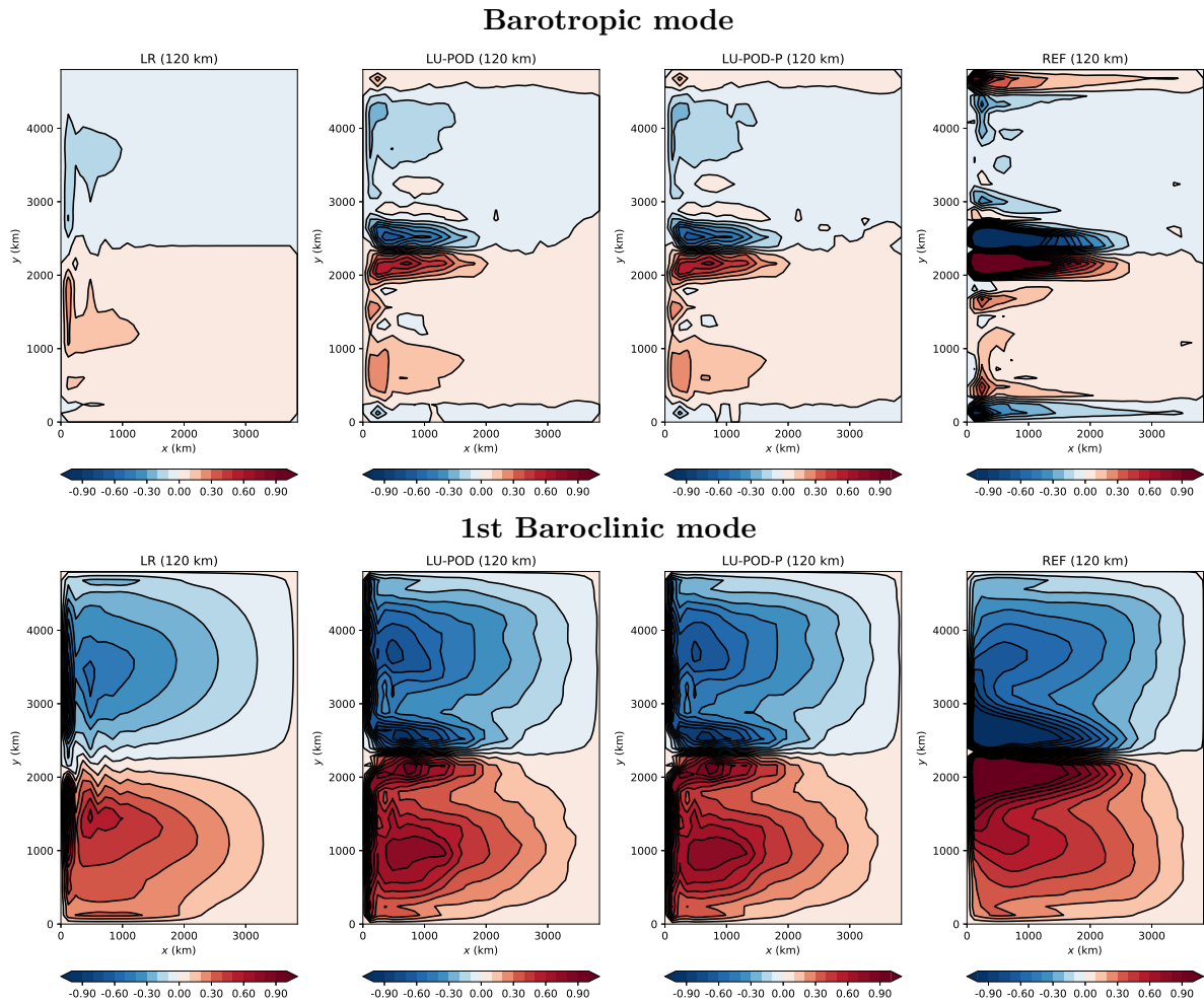
Figure 8.13 – Comparison of mean (from 60 yrs to 180 yrs) contour of vertical pressure modes for coarse-model (120 km) simulations with SST evolution. The matplotlib.colors.SymLogNorm class is used with linthresh fixed to be 0.3 and the contour interval is fixed to be 0.1 \text{ (m}^2\text{s}^{-2}\text{)} .
