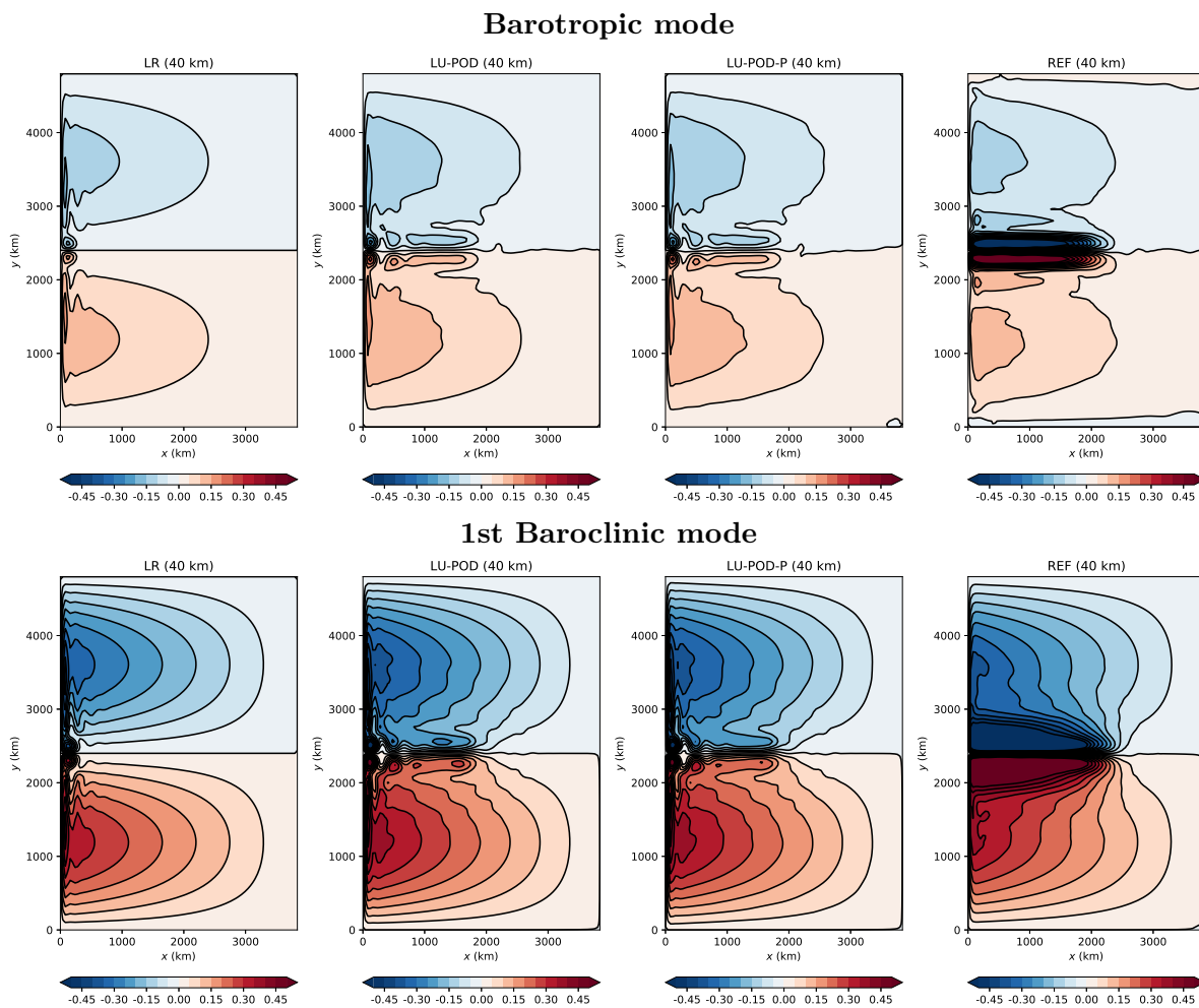
Figure 8.8 – Comparison of mean (from 60 yrs to 180 yrs) contour of vertical pressure modes for coarse-model (40 km) simulations without SST evolution. The matplotlib.colors.SymLogNorm class is used with linthresh fixed to be 0.3 and the contour interval is fixed to be 0.05 \text{ (m}^2\text{s}^{-2}\text{)} .
