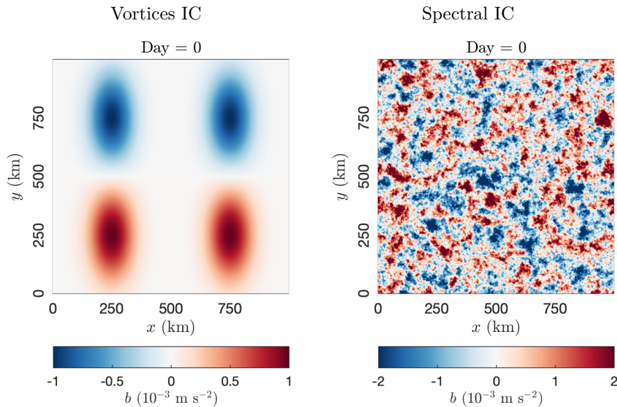
Figure 6.1 – Two initial buoyancy ( \text{m s}^{-2} ) fields. Left: a smooth field with four given vortices (cyclones in blue and anti-cyclones in red); Right: a homogeneous Gaussian field generated from a -5/3 spectrum.
