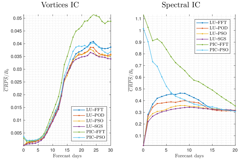
Figure 6.13 – Normalized CRPS of the spatial multivariate ensemble for each models on all time steps under both initial conditions.
