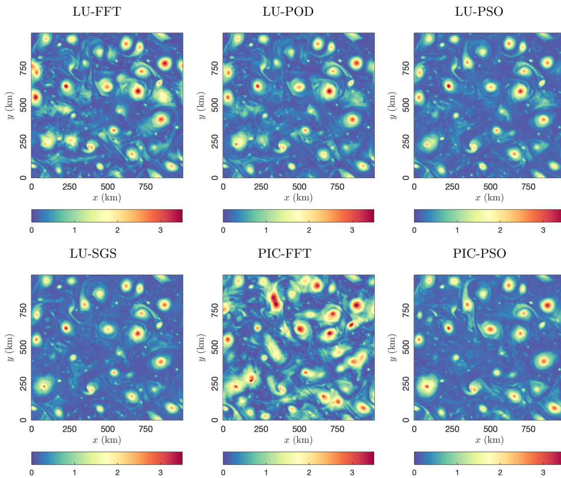
Figure 6.10 – Normalized CRPS of different random models after 10 days of advection under Spectral IC.
