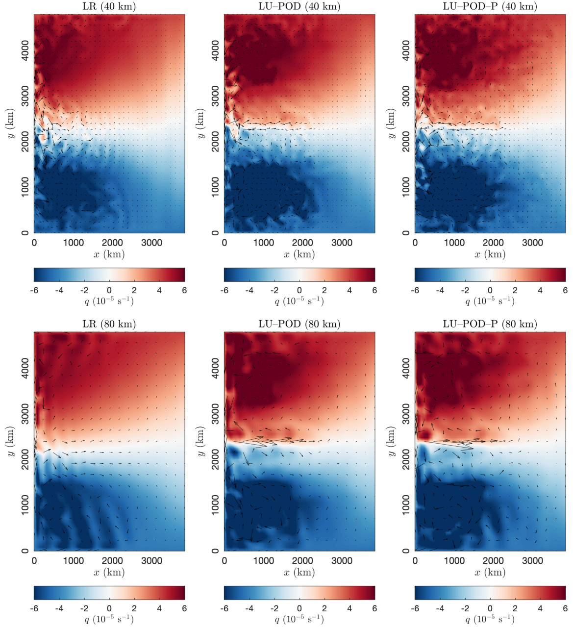
Figure 8.7 – Comparison of instantaneous (Year 60) snapshot of upper-layer PV for coarse-model simulations with SST evolution. The lengths of arrows are adjusted by a factor of 3.
