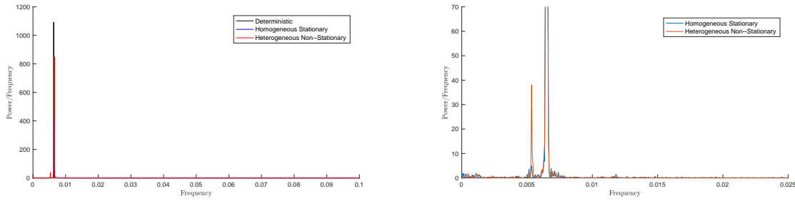
Figure 7.3 – Fourier spectra of the temporal series of a fixed grid point for the deterministic BQG, BQG-LU with homogeneous noise and BQG-LU with inhomogeneous noise; on the right zoom of the left plots.
