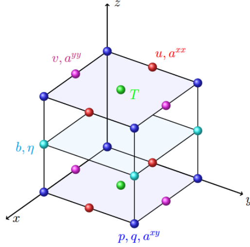
Figure 8.23 – Illustration of the discretized grid. The small-scale zonal (meridional) velocity, \dot{u} ( \dot{v} ) locates at the same position as the large-scale one, u ( v ).
