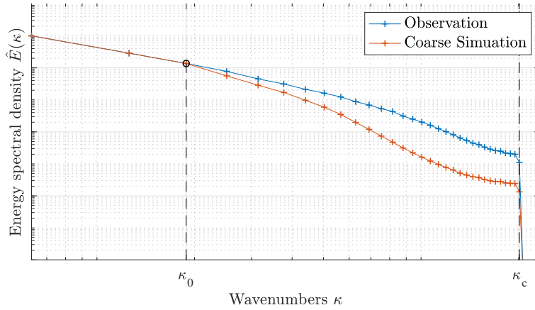
Figure 5.2 – Illustration of the time-averaged kinetic energy spectrums. The wavenumber \kappa_0 is searched as the first point where the observation and the deterministic coarse-simulation deviate, in order to estimate \gamma_0 from (5.3c).
