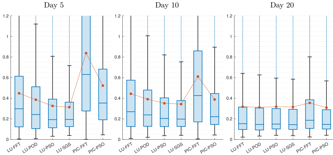
Figure 6.12 – Box plot of the normalized CRPS computed on the ensemble at each spatial points for each models at different time step of advection under Spectral IC.
