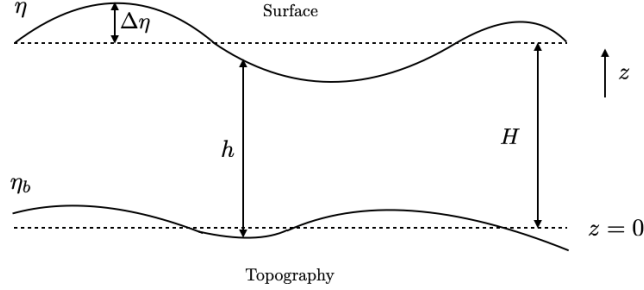
Figure 4.1 – Illustration of a single-layered shallow water system (inspired by Vallis (2017)), h is the thickness of a water column, \eta is the height of the free surface, \eta_b is the height of the bottom topography, H is the background thickness and \Delta\eta is the fluctuation of free surface height w.r.t. the background thickness. As a result, we have h = \eta - \eta_b and \eta = H + \Delta\eta .
