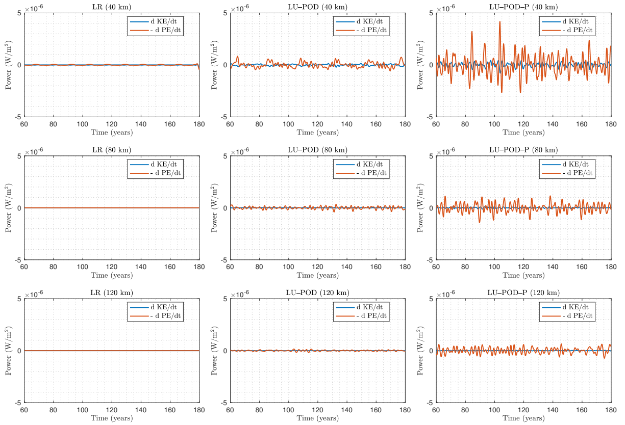
Figure 8.19 – Time series of the rate of change of KE and of the negative rate of change of PE for different coarse models (without SST). From top to bottom: 40 km, 80 km and 120 km; From left to right: LR, LU-POD, LU-POD-P.
