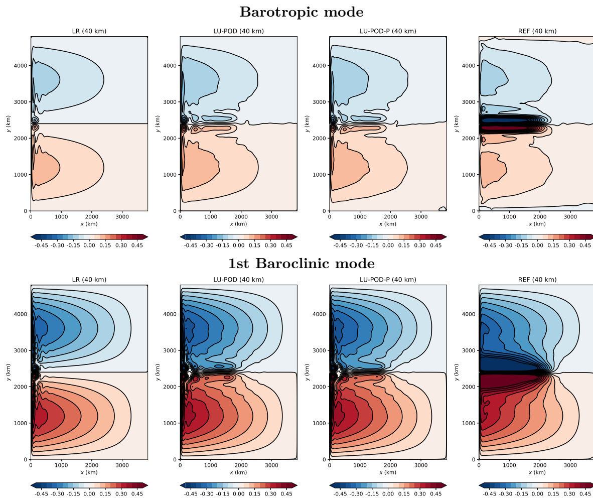
Figure 8.8 – Comparison of mean (from 60 yrs to 180 yrs) contour of vertical pressure modes for coarse-model (40 km) simulations without SST evolution. The matplotlib.colors.SymLogNorm class is used with linthresh fixed to be 0.3 and the contour interval is fixed to be 0.05 \text{ (m}^2\text{s}^{-2}\text{)} .
