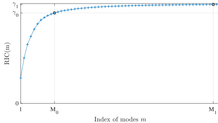
Figure 5.1 – Illustration of the spatial modes truncation for the random velocity, within the spectrum of the corresponding eigenvalues.
