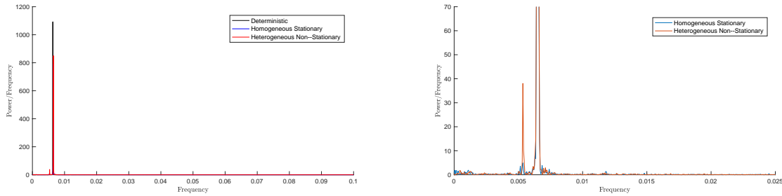
Figure 7.3 – Fourier spectra of the temporal series of a fixed grid point for the deterministic BQG, BQG-LU with homogeneous noise and BQG-LU with inhomogeneous noise; on the right zoom of the left plots.
