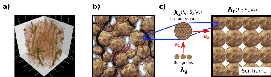
Figure 1.9 – Conceptual model of soil structure for determining macroscopic geophysical properties. (a) Computer tomography of a 100 \text{ cm}^3 soil sample from an agricultural soil (voxel size 60 \mu\text{m} , corresponding to a minimum pore width of 120 \mu\text{m} ) (from Keller et al. , 2017). (b) Conceptual illustration of a structured soil including aggregation and macroporosity created by biological activity (from Romero-Ruiz et al. , 2018). (c) Schematic representation of the upscaling of soil physical properties of structured soils from soil grains, to soil aggregates and ultimately to a soil frame. In these representations the soil is dry.
