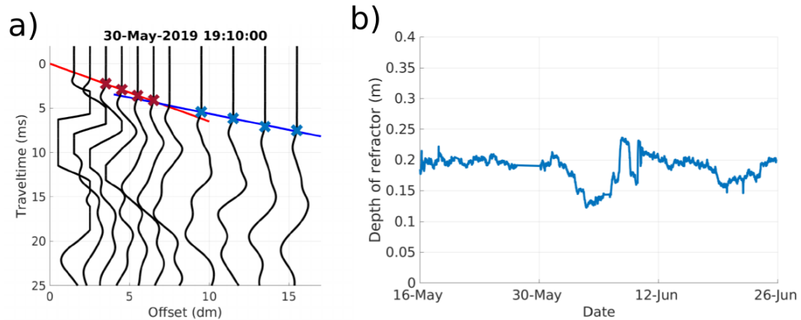
Figure 3.12 – (a) Example of seismic data recorded by the geophones at the twelve nearest offsets, at an arbitrary date, from compacted ley used to solve for the depth of the refractor. The red crosses represent the first-break picks used to calculate the P-wave velocities of the top layer (slope of the red line). The blue crosses represent the first-break picks used to calculate the P-wave velocities of the refracted wave (slope of the blue line). (b) Time series of the estimated depth of the refracting layer for the compacted ley.
