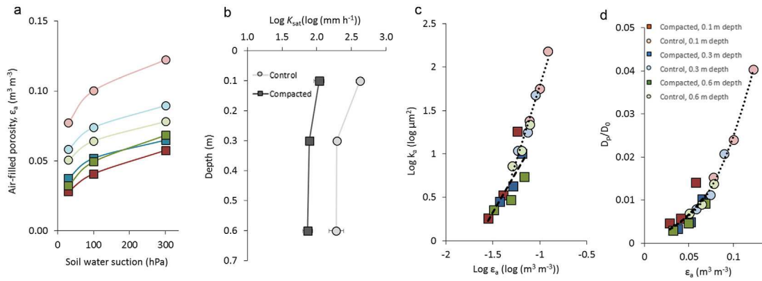
Fig. 6. Initial compaction effects on (a) air-filled porosity, \epsilon_a , at different water suctions (circles: uncompact; squares: compacted; red: 0.1-m depth, blue: 0.3-m depth, green: 0.6-m depth); (b) saturated hydraulic conductivity, K_{\text{sat}} (circles: uncompact; squares: compacted); (c) air permeability, k_a , plotted as \text{log } k_a vs. \text{log } \epsilon_a (circles: uncompact; squares: compacted; red: 0.1-m depth, blue: 0.3-m depth, green: 0.6-m depth); and (d) relative gas diffusion coefficient, D_p/D_0 , plotted as a function of \epsilon_a (circles: uncompact; squares: compacted; red: 0.1-m depth, blue: 0.3-m depth, green: 0.6-m depth). Note that the legends of Fig. 6d also apply to Fig. 6a and 6c. The data were obtained from soil cores sampled 2 wk after the compaction event. The data represent average values from the three treatments without tillage (i.e., bare soil, permanent grass, and no-till).
