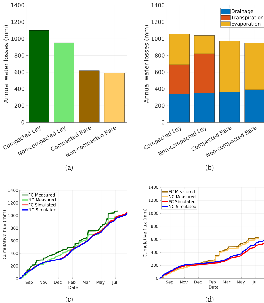
Figure 4.11 – (a) Measured total annual water losses in the top meter of soils (estimated from TDR data). (b) Total annual water losses in the top meter of soils resulting from the Hydrus simulations. The different soil fluxes are marked with different colors for each soil case. (c) Measured and simulated cumulative total water losses as a function of time for compacted and non-compacted ley. (d) Measured total water losses and simulated evaporation as a function of time for compacted and non-compacted bare soil. The time axis goes from the middle of 2017 to the middle of 2018
