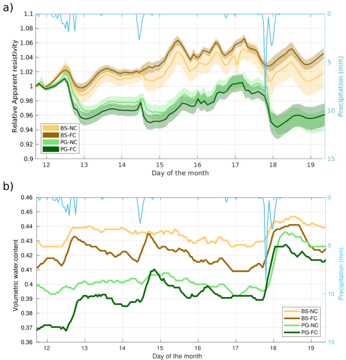
Figure 2.9 – (a) Relative time-lapse changes in electrical resistivity of the first level of the Wenner array for bare soil compacted (BS-FC), bare soil non compacted (BS-NC), permanent grass compacted (PG-FC) and permanent grass non compacted (PG-NC). (b) Volumetric water content estimated from TDR measurements at 20 cm depth, located in the same plots as in (a).
