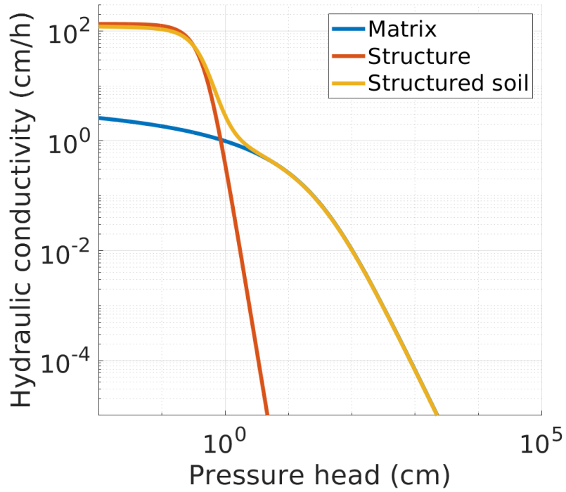
Figure 1.10 – Hydraulic conductivity function of structured soils as the superposition of soil matrix and soil structural pores. We used the parametric model of van Genuchten (1980) to model the hydraulic conductivity functions. The properties for soil matrix are: \alpha_{sm} = 0.02 \text{ cm}^{-1} , n_{sm} = 1.15 , K_{s_{sm}} = 3 \text{ cm/h} , w_{sm} = 0.96 \text{ cm}^3/\text{cm}^3 . The properties of the soil macropores are \alpha_{mac} = 2 \text{ cm}^{-1} , n_{mac} = 3 , K_{s_{mac}} = 2500 \text{ cm/h} , and w_{sm} = 0.04 \text{ cm}^3/\text{cm}^3 .
