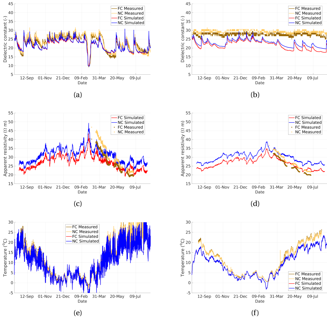
Figure 4.7 – Modeled and measured dielectric constant of compacted and non-compacted bare soil at (a) 10 cm and (b) 40 cm depth. Modeled and measured electrical resistivity of compacted and non-compacted bare soils using (c) j=1 and (d) j=3 in the Wenner-Schlumberger array. Modeled and measured temperature of compacted and non-compacted bare soils at (e) 10 cm and (f) 40 cm depth. The time axis goes from the middle of 2017 to the middle of 2018.
