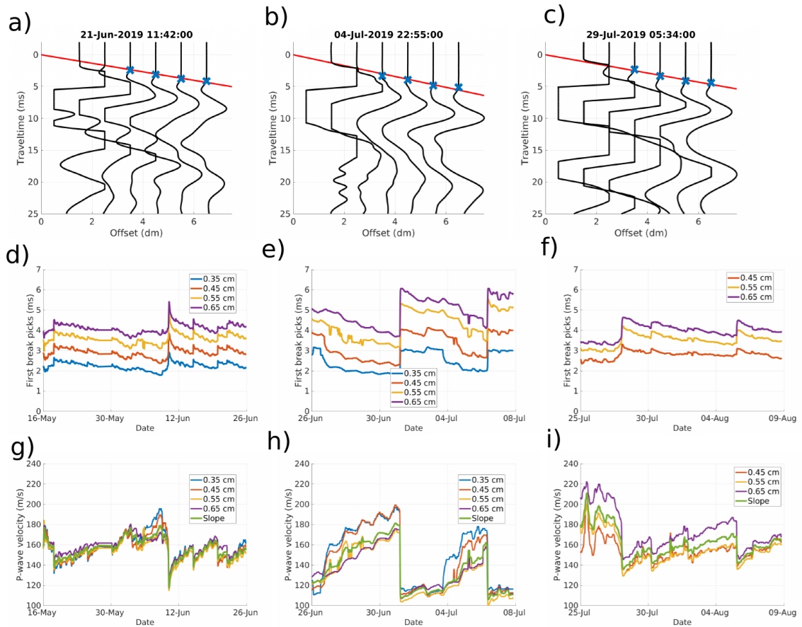
Figure 3.10 – Examples of seismic data recorded by the geophones at the six nearest offsets at an arbitrary date from (a) compacted ley, (b) non-compacted ley and (c) compacted bare soil. The blue crosses correspond to the first-break picks used to calculate the P-wave velocities from to the slope of the red line. Time-series of the picked first-break times for different offsets in the (d) compacted ley, (e) non-compacted ley and (f) compacted bare soil. Time series of the calculated P-wave velocities for different offsets along with the velocity calculated with the slope method for (g) compacted ley, (h) non-compacted ley and (i) compacted bare soil.
