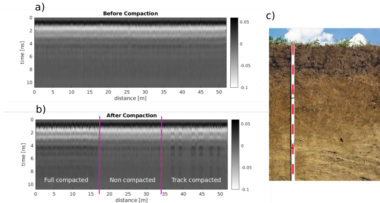
Figure 2.5 – GPR spatial identification of compacted zones in a compaction field experiment (described by Keller et al., 2017 ) in Zürich, Switzerland. (a) Data collected before the compaction event. (b) Data collected after the compaction event at the same location. (c) Soil profile from a non-compacted zone in the experimental field. The red and white color in the ruler alternate every 10 cm.
