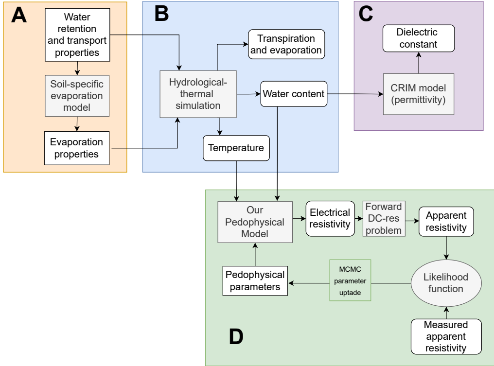
Figure 4.2 – Flowchart for hydrogeophysical forward and inverse modeling including soil evaporation constrains. The flowchart is divided in blocks containing different modeling steps involved in the coupled model. In A, water retention and transport properties are used to calculate treatment-specific evaporation properties. The water retention, transport and evaporation properties are used to perform a hydro-thermal simulation with Hydrus-1D resulting in soil water fluxes, water content and temperature. In C, the water content time-series are used with the CRIM model to model dielectric constant for comparison with TDR data. The inverse modeling of the electrical data is presented in D. The water content and temperature are used with the new pedophysical model to compute electrical resistivity profiles that are in turn used to compute apparent electrical resistivity. The pedophysical electrical properties are inferred using MCMC.
