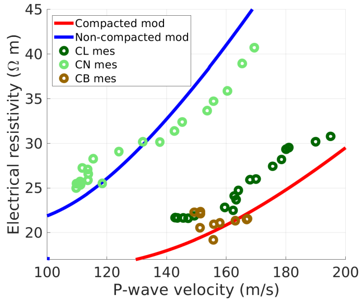
Figure 5.1 – Modeled and measured apparent resistivity against seismic velocities as a function of water content. The measured P-wave velocities correspond to the velocities of the first layer Chapter 3, while the apparent resistivities correspond to the j=1 in the Wenner-Schlumberger array in Chapter 4.
