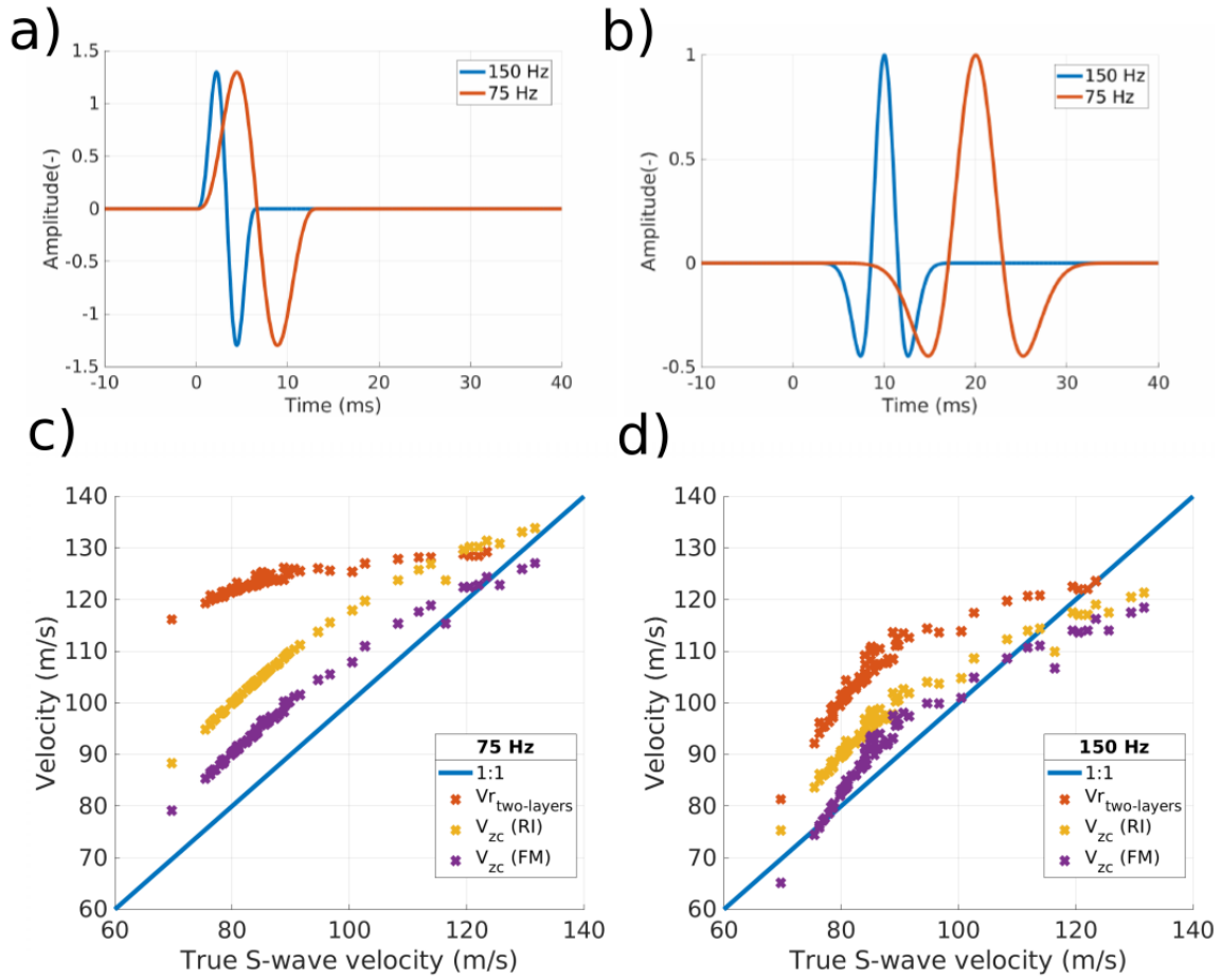
Figure 3.13 – (a) Fuchs-Müller and (b) Ricker wavelets with central frequencies of 75 and 150 Hz. Comparison of true vs. estimated S-wave velocities in a two-layer media for two different source wavelets and two different central frequencies: (c) 75 Hz and (d) 150 Hz. In (c) and (d), the true R-wave velocity ( V_r ) is shown for comparison purposes.
