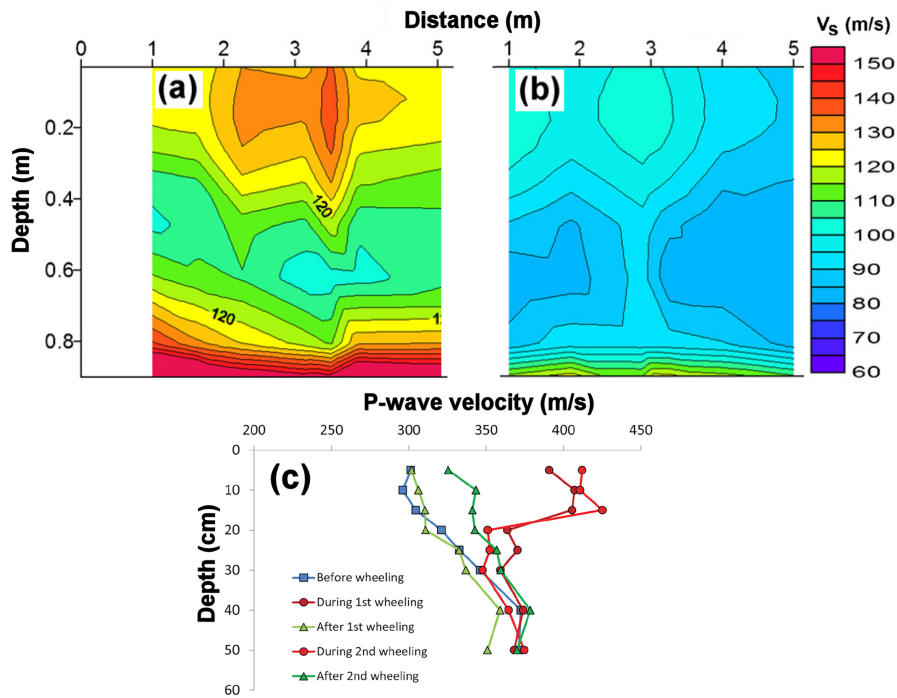
Figure 2.6 – The sensitivity of seismic measurements to soil compaction and load: S-wave sections from Multichannel Analysis of Seismic Waves (MASW) deduced from a compacted zone (a) and a non-compacted zone (b), note lower S-wave velocities for the non-compacted soil (from Donohue et al. , 2013); and (c) p-wave velocity with depth measured in a wheeling experiment marking changes during load application and after passage of the wheel (from Keller et al. , 2013b).
