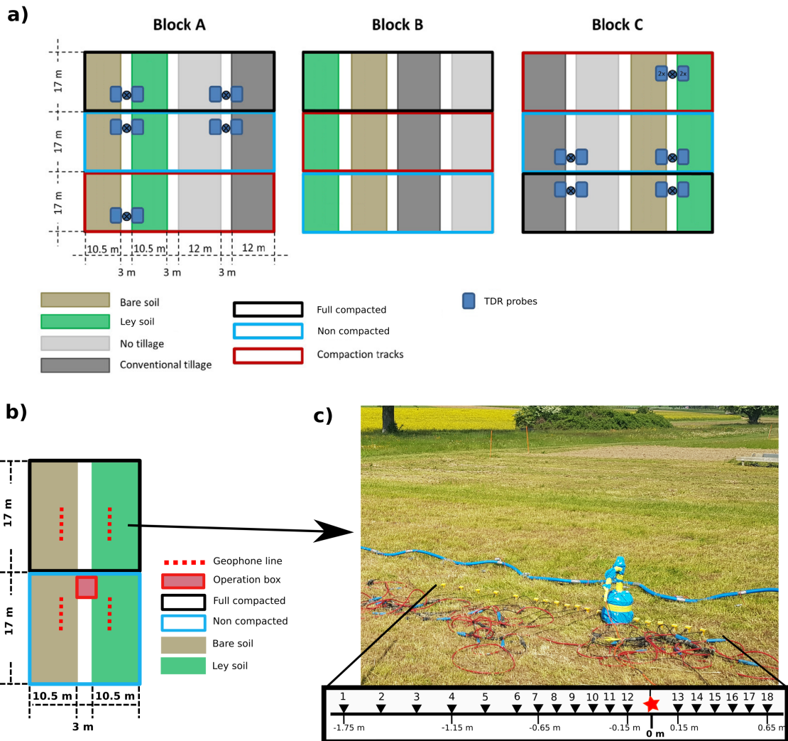
Figure 3.2 – (a) Schematic representation of the soil compaction experiment showing the different compaction treatments and post-compaction management strategies at the SSO (adapted from Keller et al., 2017 ). (b) Schematic representation of the seismic lines deployed in block A. (c) Seismic monitoring layout established in the compacted ley.
