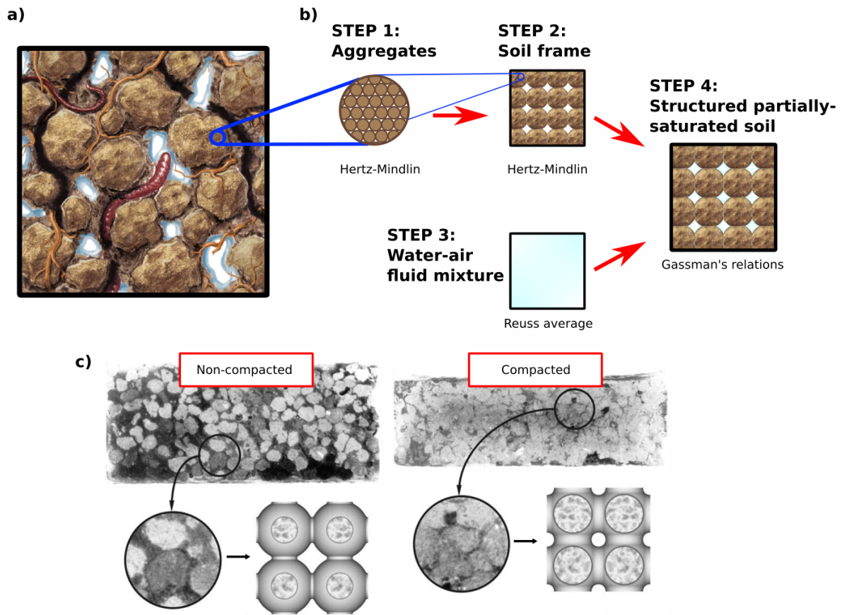
Figure 3.1 – Conceptualization of soil structural elements and their integration within a self-consistent pedophysical model of macroscopic elastic properties. (a) Schematic representation of a structured soil displaying aggregation (taken from Romero-Ruiz et al. , 2018). (b) Sketch of the four mixing steps used to predict the elastic properties of partially-saturated structured soils with the model type used at each step. (c) Schematic representation of aggregate geometries as conceptualized in step 2 (modified from Ghezzehei and Or , 2003).
