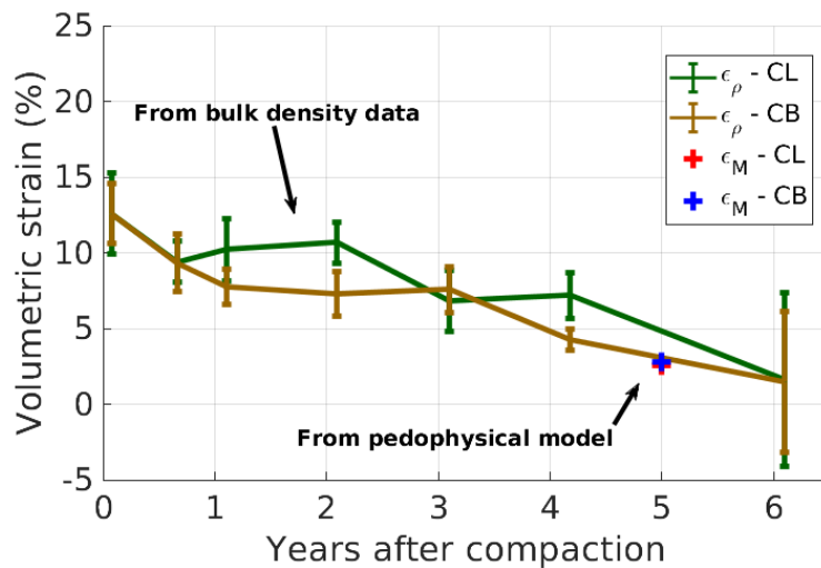
Figure 3.8 – Comparison of soil volumetric strain derived from dry bulk density data ( \epsilon_\rho ) as a function of the time since the compaction event and the volumetric strain estimated from inferences of axial strains obtained from the pedophysical model and seismic data ( \epsilon_M ). The volumetric strains from bulk densities and pedophysical model were obtained by comparing compacted ley (CL) and compacted bare soil (CB) with non-compacted ley at the same time after the experimental compaction event.
