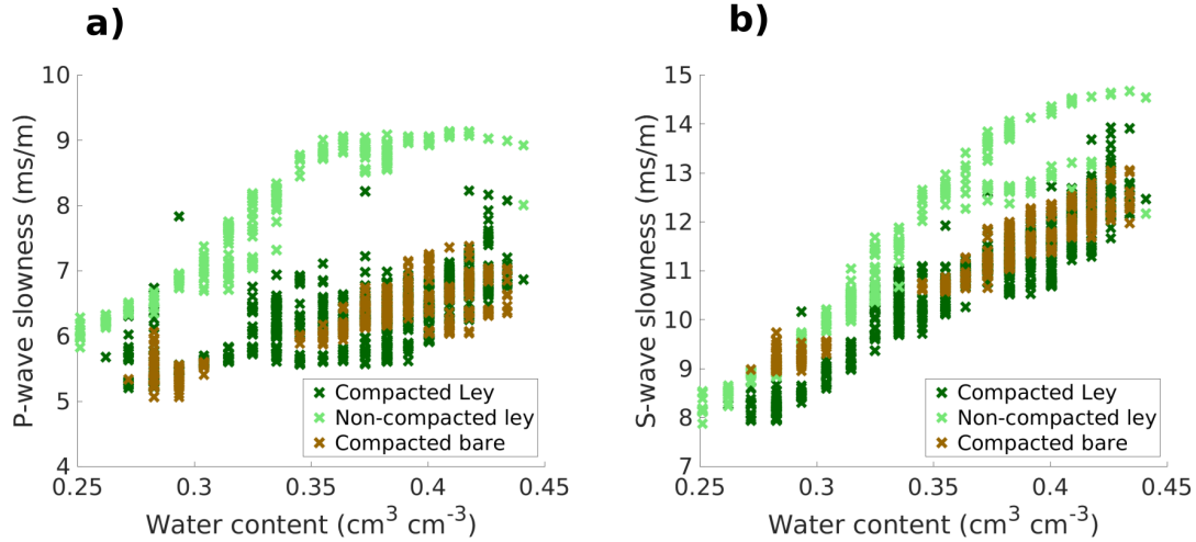
Figure 3.4 – Scatter plot of (a) P-wave and (b) S-wave slowness as a function of water content for all soil treatments.
