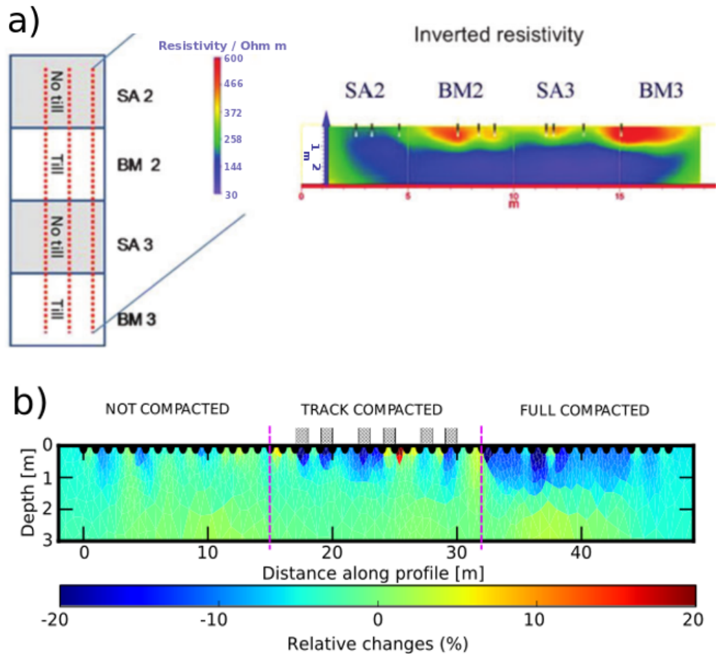
Figure 2.4 – (a) Experimental set-up of DC-resistivity measurements after the tillage experiment by Rossi et al. (2013a), soil electrical resistivity tomogram from data taken on one of transects in that cross the alternating tillage (BM2 and BM3) and non-tillage (SA2 and SA3) management regions. (b) Relative changes (before and after soil compaction) in inferred electrical resistivity of a soil ( Keller et al. , 2017). Gray rectangles indicate track passages and the full compacted part was made by consecutive passages of tracks next to each other.
