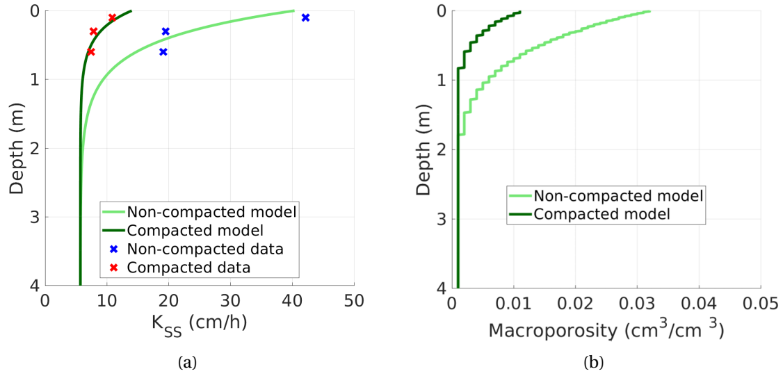
Figure 4.5 – (a) Measured and modeled saturated hydraulic conductivity as a function of soil depth for compacted and non-compacted soils. (b) Estimated macroporosity as a function of soil depth for compacted and non-compacted soils.
