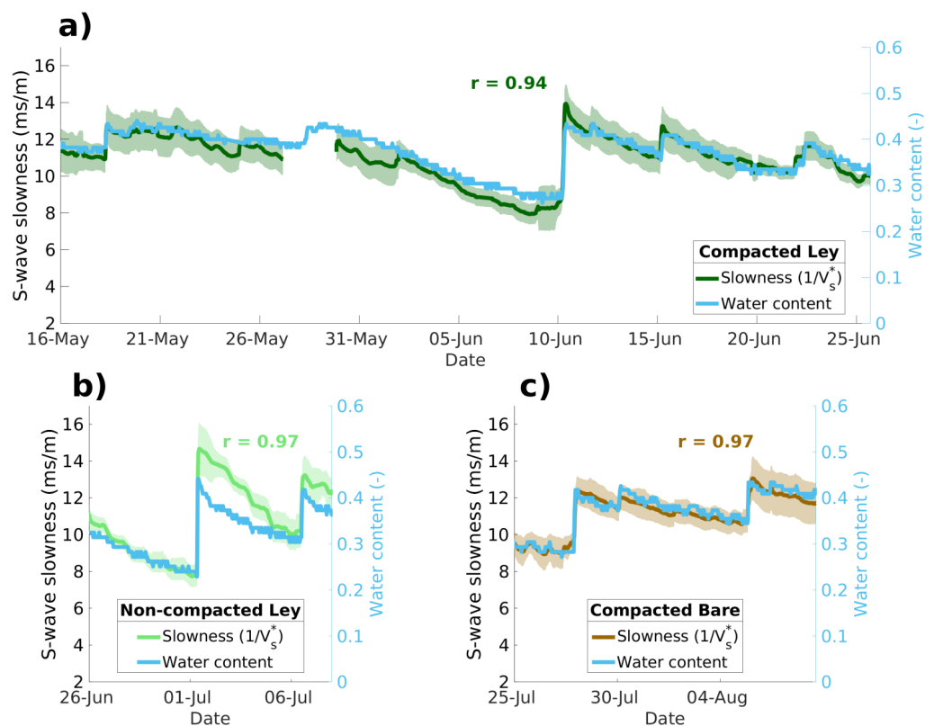
Figure 3.3 – Time-series of estimated S-wave slowness and water content for: (a) full compacted ley, (b) non-compacted ley, and (c) full compacted bare soil. Note that slowness and water content correspond to different time-periods for the different soil treatments.
