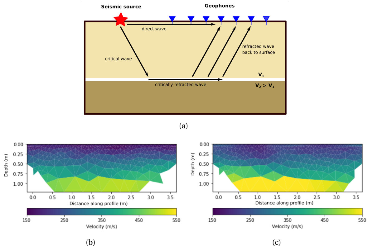
Figure 1.7 – Seismic refraction imaging. (a) Schematic representation of the seismic refraction ray-path. Inverted P-wave velocity sections from seismic refraction surveys collected in (b) non-compacted and (c) compacted bare soil with a loamy texture in the soil compaction experiment presented by Keller et al. (2017).
