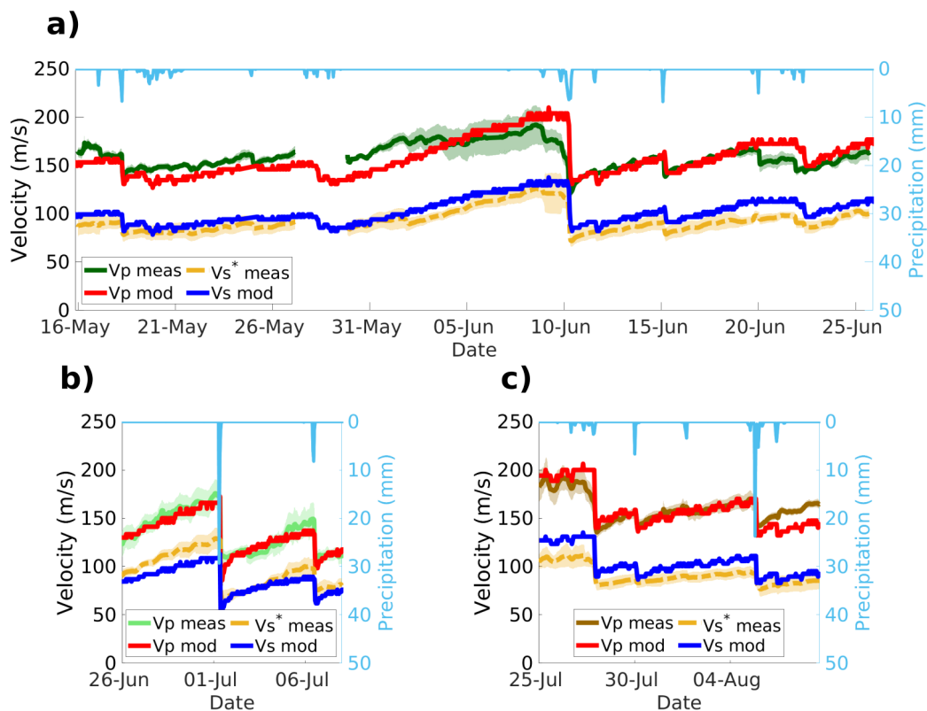
Figure 3.5 – Time series of modeled (mod) and measured (meas) P-wave and S-wave velocities for (a) compacted ley, (b) non-compacted ley and (c) compacted bare soil along with precipitation data (light blue right hand axes).
