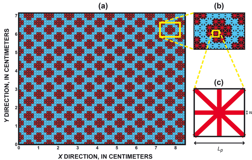
Figure 2.7 – (a) Diagram illustrating a bimodal pore network model (PNM) consisting of a pipe lattice with a given porosity (blue) between accumulations of zeolite grains (red) with (c) an internal porosity. From Day-Lewis et al. (2017).
