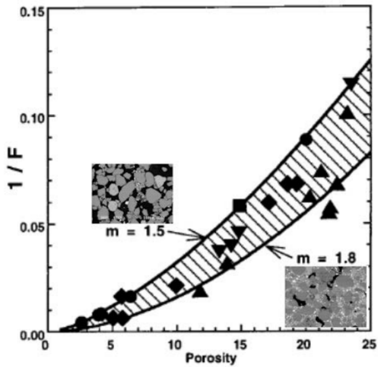
Figure 2.3 – Relationship between the inverse of the electrical formation factor and porosity in Archie’s law (Equation 2.1). Two values of the cementation exponent are shown to illustrate how it affects the formation factor: m = 1.5 has a more connected pore network than m = 1.8 as shown in the photographs, where the pore space is black and the solid phase is gray. Modified from Revil and Cathles (1999)
