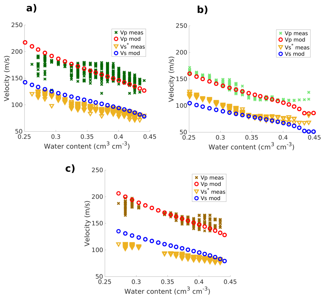
Figure 3.6 – Scatter plot of modeled and measured P-wave and S-wave velocities as functions of soil water content for (a) compacted ley, (b) non-compacted ley and (c) compacted bare soil.
