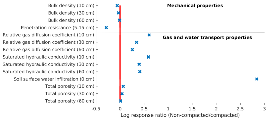
Figure 1.3 – Metrics of non-compacted soil structure relative to compacted soil structure. Data are from a soil compaction field experiment presented by Keller et al. (2017) . Data from compacted soils were measured shortly after experimental compaction. The numbers in the parenthesis indicate the soil depth for soil samples. The values of soil penetration resistance are averaged between 5 and 15 cm. The horizontal value presents the log 10 of the ratio between values from non-compacted and compacted soils.
