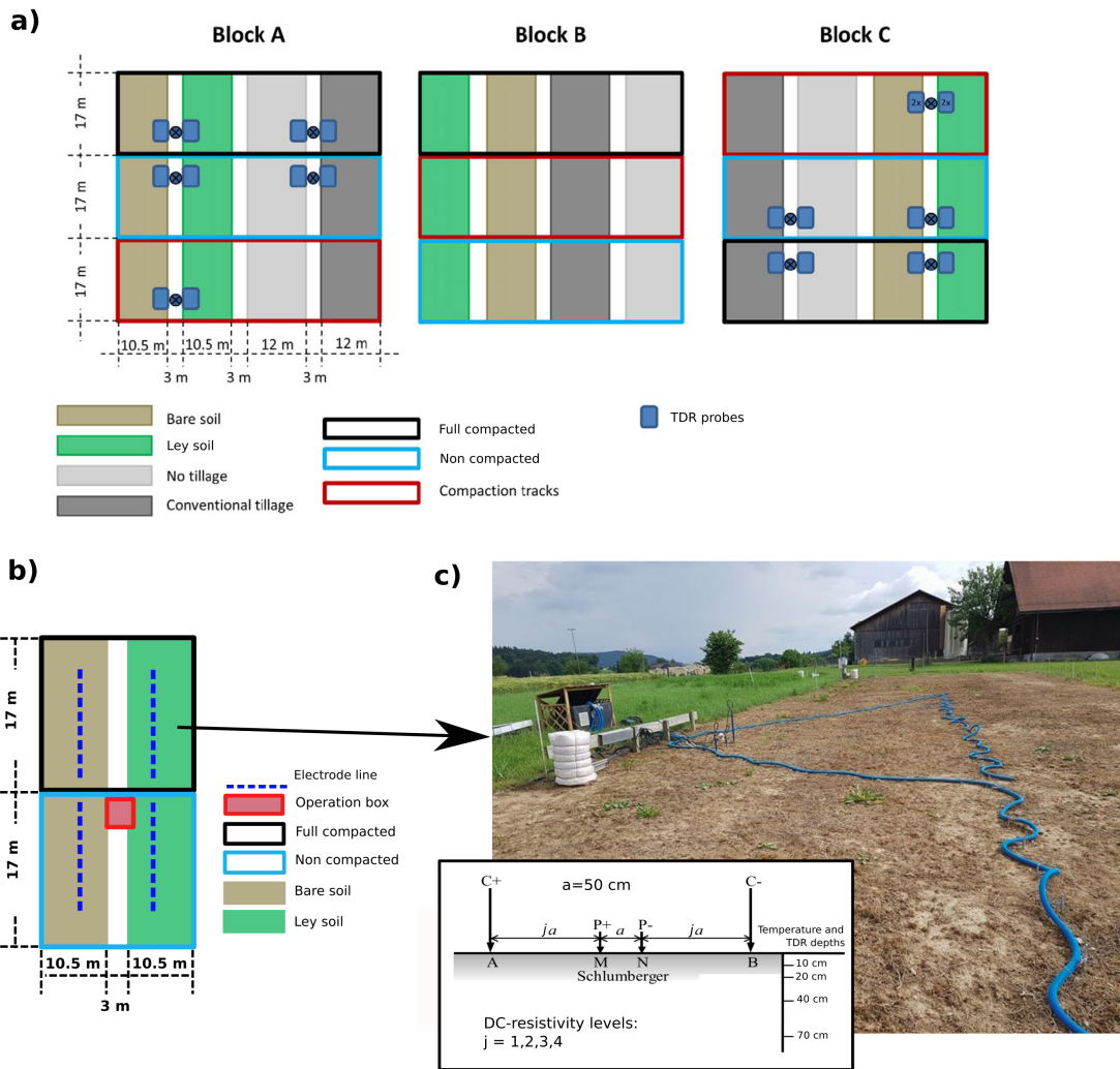
Figure 4.3 – (a) Schematic representation of the soil compaction experiment showing the different compaction treatments and post-compaction management strategies at the Soil Structure Observatory. (b) Schematic representation of the DC-resistivity lines deployed in the block A. (c) DC-resistivity line located in the bare soil.
