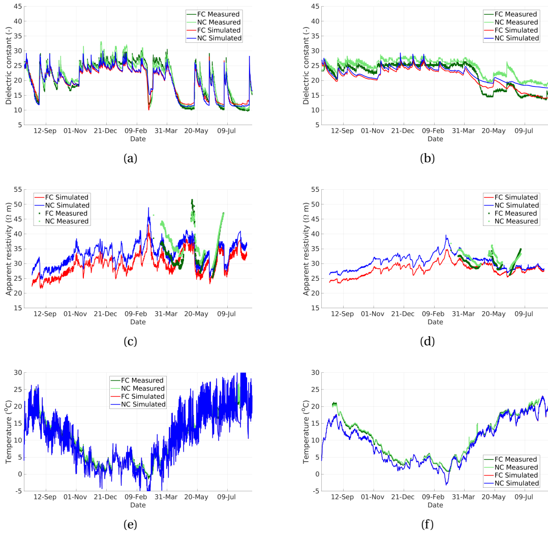
Figure 4.8 – Modeled and measured dielectric constant of compacted and non-compacted ley soils at (a) 10 cm and (b) 40 cm depth. Modeled and measured electrical resistivity of compacted and non-compacted ley soils using (c) j=1 and (d) j=3 in the Wenner-Schlumberger array. Modeled and measured temperature of compacted and non-compacted ley soils at (e) 10 cm and (f) 40 cm depth. The time axis goes from the middle of 2017 to the middle of 2018.
